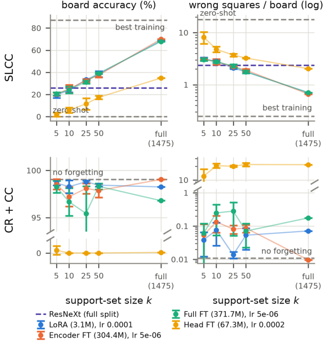
Figure 6. Few-shot adaptation of ChessQueries from ChessReD + ChessCog to the SLCC domain. Top: accuracy on the target (SLCC), bounded by the zero-shot floor and our best training’s ceiling (87.1% board accuracy, see Tab. 1); the colored dashed line marks ChessReD’s ResNeXt baseline trained on the full SLCC split (26.0%, Tab. 1), matched by a LoRA on 10 frames. Bottom: forgetting is measured via the mean performance retained on the source domains (ChessReD + ChessCog). Full protocol details: Sec. C.
