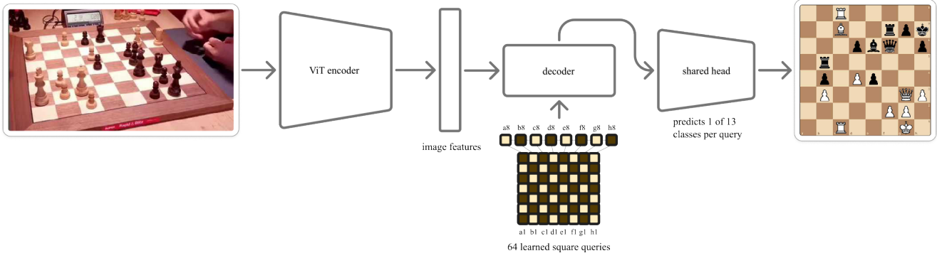
Figure 2. ChessQueries architecture. A ViT-L encoder turns the input image into patch tokens. Sixty-four learned square queries — one per board square — cross-attend to those tokens, and a single shared linear head maps each decoded query to one of 13 classes (six piece types, times two colors, plus empty square), yielding the full 8 \times 8 board in one forward pass.
