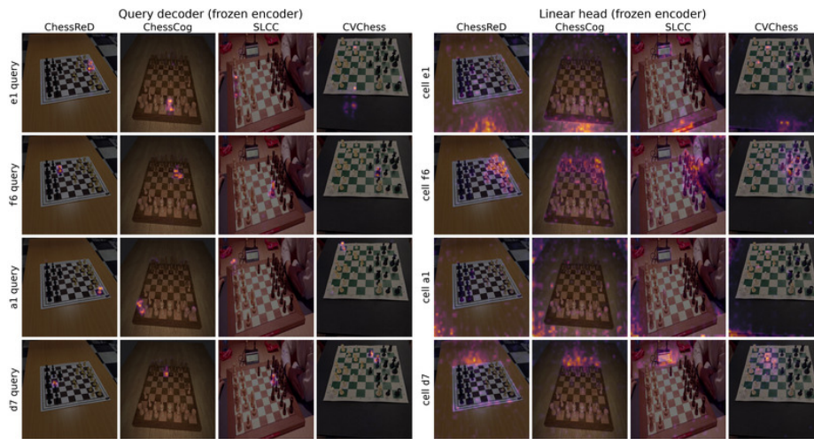
Figure 13. Attention with a frozen encoder (Tab. 4, bottom block). Left: the query decoder’s cross-attention still localizes each square on frozen DINOv2 features — the decoder computes the image-to-board correspondence itself. Right: the encoder cell attention available to the linear head is diffuse and largely off-board, with no consistent per-square localization, matching its majority-class-floor accuracy.
