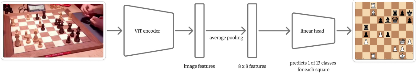
Figure 7. Architecture of the linear-head baseline compared against in Tab. 4. The 64 square queries and the cross-attention decoder of Fig. 2 are removed, and replaced by average pooling and a simple linear head.
