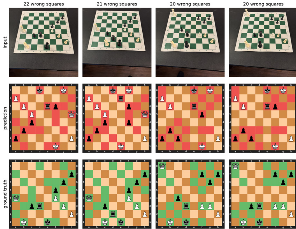
Figure 10. The four CVChess positions where our model performs worst. The failures appear from the default viewpoint, facing the white pieces: the model reads those boards essentially upside down – 2–4 wrong squares once the ground truth is turned 180°. We also observe impossible outputs such as two white kings. Figure 11 shows the first 2 positions seen from different viewpoints and parsed correctly.
