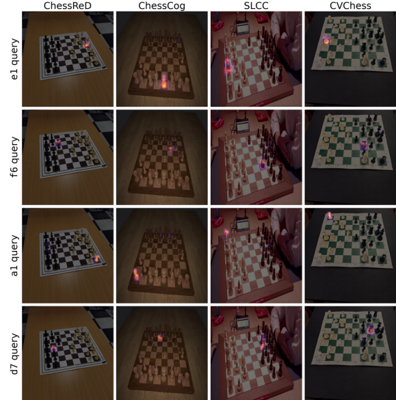
Figure 4. Query attention for 4 separate square queries.
