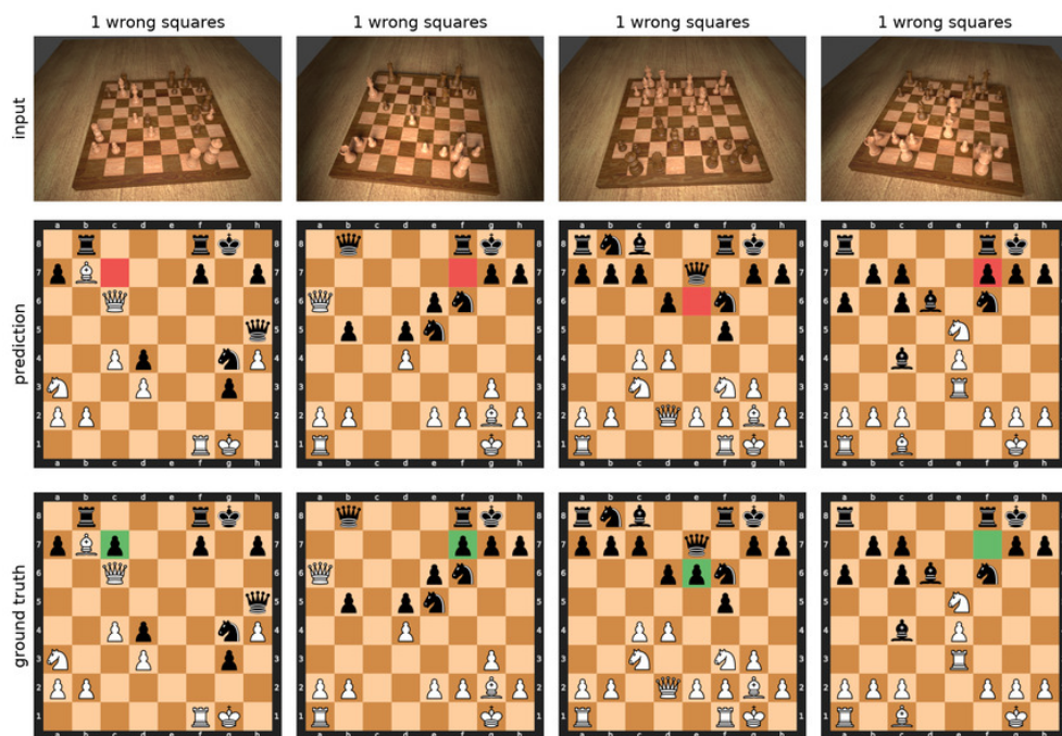
Figure 9. The four ChessCog test images where our model performs worst: a single wrong square each on this near-saturated synthetic domain, with the mistaken piece heavily occluded.
