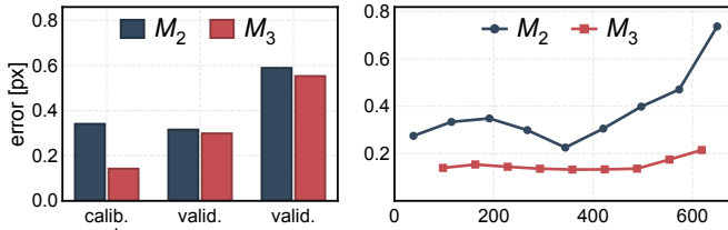
Fig. 4: Distortion-order selection on Rig-A. Left: mean corner error [px] of both candidates on the calibration set and the validation views. Right: per-view residual against the radial distance r from the principal point, over the observed range.
