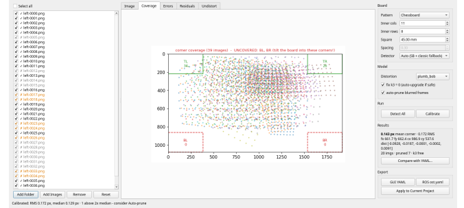
Fig. 6: Interface on Rig-A after calibration. Left: image list, with images rejected at Stage 1 greyed out and those rejected at Stage 2 marked in orange. Center: calibration points and corner-zone counts. Right: board and model settings with the estimated parameters. The status bar reports the residual and the number of views exceeding \kappa\bar{e} .
