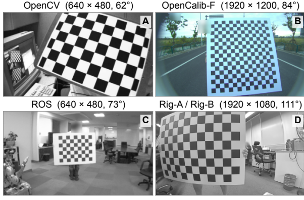
Fig. 2: The four camera models evaluated, 62° to 111° diagonal field of view: (A) OpenCV, 9 × 6 board; (B) OpenCalib-F, 17 × 15, the only outdoor scene; (C) ROS, 8 × 6; (D) Rig-A/Rig-B, 11 × 8, captured on our own rig.
