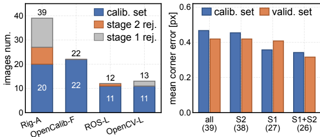
Fig. 3: Image selection. Left: images kept and rejected per stage; right stereo cameras omitted (identical to left). Right: calibration and validation mean corner error [px] of four Rig-A sets, \mathcal{M}_2 .
