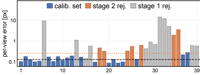
Fig. 5: Per-view residual of all 39 Rig-A images, under the final model and colored by selection result. Dashed: median of the calibration set; dotted: rejection threshold \tau = 2\bar{e} .
