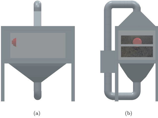
Fig. 2. Design drawing of the laboratory test bench. The system consists of a chamber with a camera on one side and a monitor on the opposite side, which can display various backgrounds. The camera is illustrated with a red camera symbol, and an image is displayed on the screen. The dust is circulated using a ventilation system. As a result, the dust density can be controlled with a fan. (a) Front view. (b) Side view.
