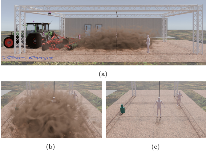
Fig. 4. Overview of the outdoor test field with gate for mounting of sensors. A tractor can drive through the gate to cultivate the field. This allows dust-free and dusty sensor data to be recorded. (a) Side view. (b) Sensor view with dust; (c) Sensor view without dust.
