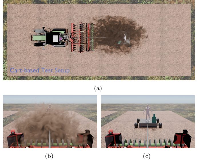
Fig. 5. Overview of the cart-based test setup with a cart attached to a tractor implement using a wire rope. Certified test objects can be mounted on the carrier. (a) Top-down view. View from the perspective of the sensors mounted to the tractor’s rear window with dust (b) and without dust (c)
