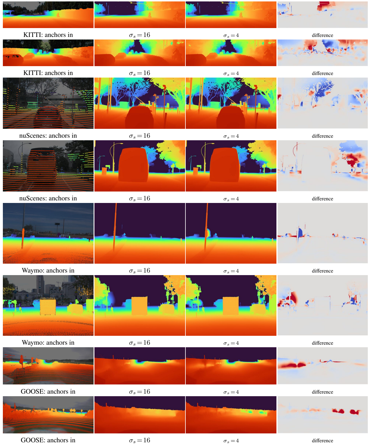
Figure 9: Solver sensitivity, two frames per dataset: the anchors given to the solver, depth at the default \sigma_s = 16 , at \sigma_s = 4 , and their signed difference (blue nearer, red farther, grey unchanged, each panel on its own scale). At \sigma_s = 4 the correction concentrates into blobs at individual anchors instead of travelling along surfaces — the 21–33% RMSE it buys is paid for in surface damage. NYU is omitted: its two settings differ by under a centimetre.
