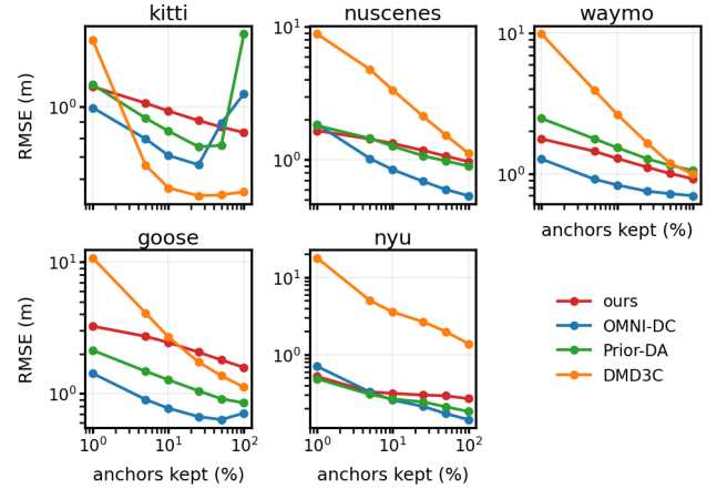
Figure 8: Anchor-density sweep.
