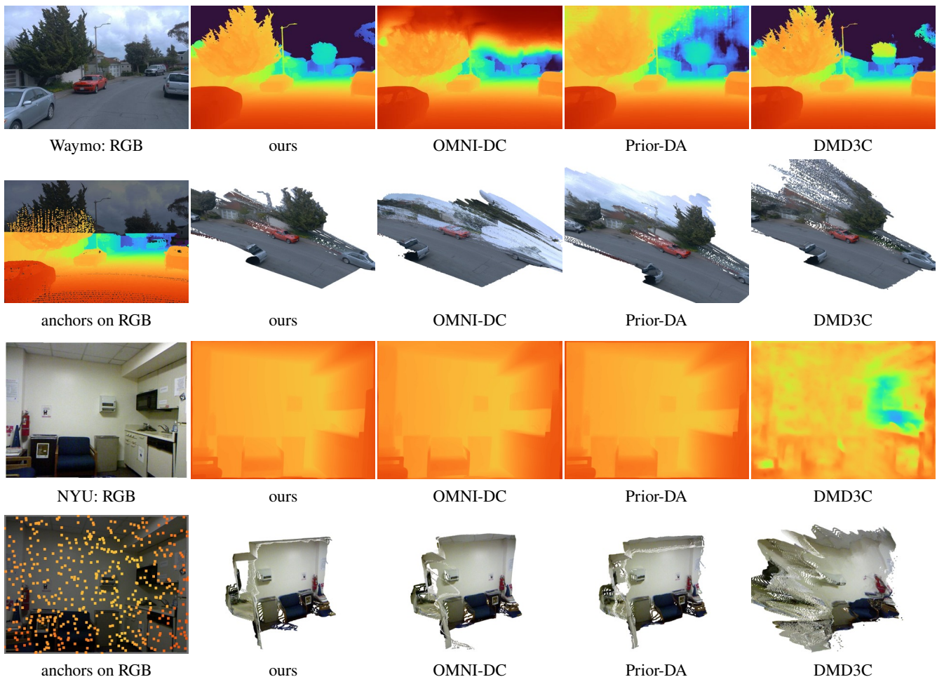
Figure 12: The same depth maps, turned back into 3D. For each scene the upper row is the input image and each method’s depth map; the lower row is the anchors the solver was given, drawn over the image, and each depth map re-projected into a coloured point cloud, all seen from a direction the camera never occupied ( 35^\circ azimuth, 18^\circ elevation). From the original viewpoint all four look alike by construction, since each is consistent with the same image. The depth maps are indeed hard to separate — but only ours re-projects to continuous surfaces. On Waymo the baselines smear the buildings and trees behind the road into sheets of stray points that hang over the scene; on NYU, where OMNI-DC and Prior-DA are metrically ahead of us, the room still resolves for all three and only DMD3C disintegrates. This is what the normal-dispersion column measures, and what a downstream consumer of the depth map receives.
