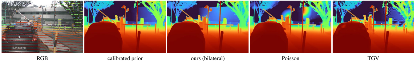
Figure 4: Solver comparison on a sparse-anchor nuScenes crop. All methods start from the same calibrated prior and anchors. Pixel-wise Poisson and TGV produce anchor-centred surface bumps, whereas FounRef shares corrections on a coarse bilateral grid. Depth panels share the [1, 50] m range.
