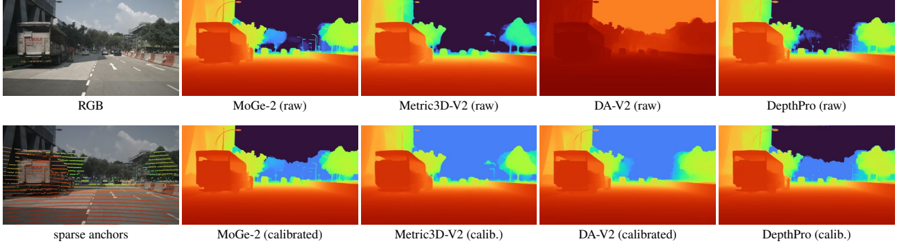
Figure 2: Global calibration of four priors on the same frame. Top: raw predictions use incompatible depth scales; DA-V2 is relative. Bottom: after fitting the same sparse anchors, all priors share a metric scale while preserving their edges and relative layout. All depth panels use the 0–80m range. Pixels a prior marks invalid (sky) are drawn at the far end (MoGe-2 provides an invalid map, while depth pro predicts them at 10,000m).
