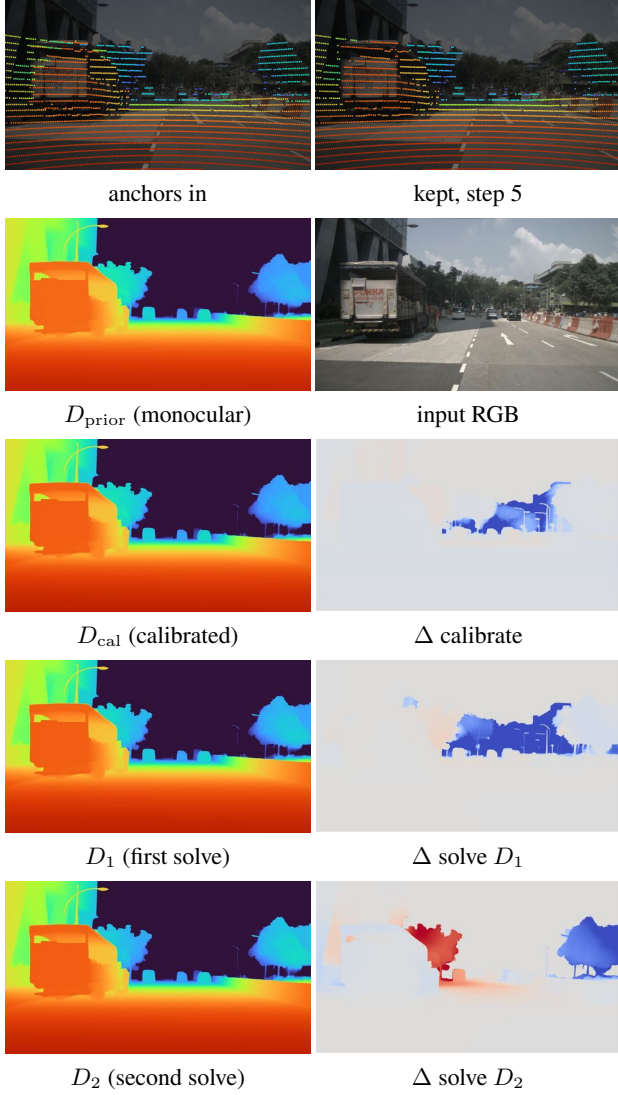
Figure 7: The pipeline on one nuScenes frame, by row: left the state after a step, right what that step changed (blue nearer, red farther, grey unchanged, each panel on its own scale). Top: anchors in, and what survives the anchor filter (4.7% removed), dilated for legibility.
