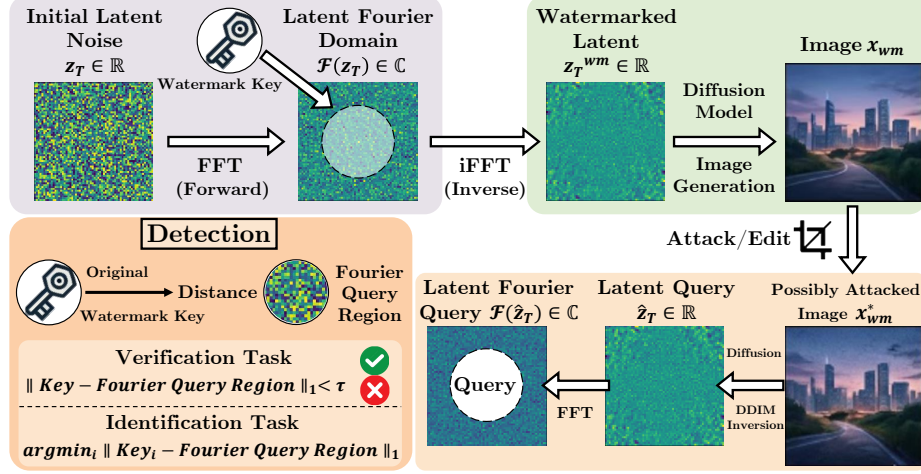
Fig. 1: Representative generation-time z_T -Fourier watermarking pipeline used in the case studies: a keyed Fourier pattern is inserted into the initial noise, propagated through diffusion generation, recovered from an optionally transformed query via DDIM inversion, and compared with reference keys for verification or closed-set identification. Reproduced from [18], which is itself adapted from [15]. The diagram does not represent post-hoc optimization, spatial- z_T , z_0 , or pixel-domain methods, and the optional transformation is illustrative rather than a robustness claim.
