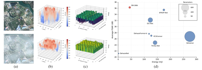
Figure 1: Visualization of haze-induced degradation and spiking responses. (a) Remote-sensing patch under clear (top) and hazy (bottom) conditions. (b) 3D intensity surface plots of the patches. (c) LIF membrane potentials over neuron index and simulation step. (d) PSNR versus energy consumption on RICE-2; bubble size indicates parameter.
