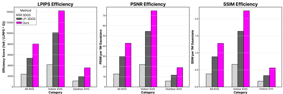
Figure 3: Efficiency scores on Mip-NeRF 360 across three metrics ( 10^9/(\text{LPIPS} \times \#G) , \text{PSNR}/\#G , \text{SSIM}/\#G ). LinearMask-GS achieves the highest score on all three, indicating superior perceptual quality per Gaussian.
