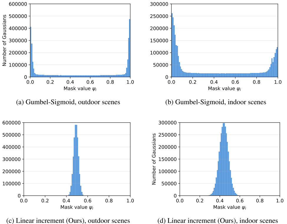
Figure 1: Mask \psi_i distribution at the end of mask training, aggregated separately over MipNeRF 360’s outdoor (5 scenes) and indoor (4 scenes) sets. (a, b) Gumbel-Sigmoid produces a two-peaked distribution pinned at 0 and 1; the fraction above \psi = 0.5 is scene-dependent ( \sim 52\% outdoor, \sim 40\% indoor), reflecting that which side each mask lands on is unrelated to importance. (c, d) Linear increment yields a unimodal distribution near \psi = 0.5 (mean \sim 0.44 indoor, \sim 0.49 outdoor), so the relative order of mask values is preserved and the top- \rho N pruning in Eq. (9) operates on a stable ranking.
