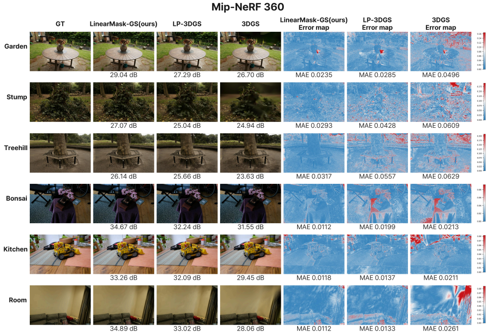
Figure 7: Per-pixel qualitative comparison on the six Mip-NeRF 360 scenes not shown in the main paper’s Figure 2. Each row shows one scene; columns from left to right show the ground truth, the rendered images from LinearMask-GS (ours), LP-3DGS, and 3DGS, followed by per-pixel absolute error maps for the same three methods. Per-image PSNR (dB) is reported below each render and per-image MAE below each error map; error maps use a scene-specific blue-to-red colormap (low to high absolute error).
