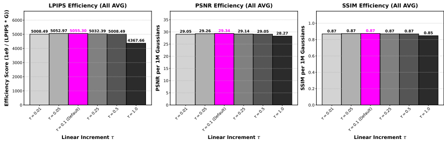
Figure 3: Sensitivity to \tau . Efficiency score under varying slope \tau on Mip-NeRF 360. The default \tau = 0.1 (highlighted) achieves the best LPIPS-based efficiency score.
