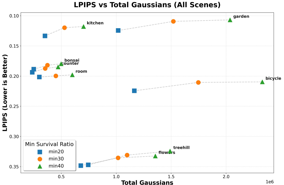
Figure 8: Effect of the minimum-survival ratio \rho on Mip-NeRF 360: per-scene LPIPS vs. number of Gaussians for \rho \in \{0.20, 0.30, 0.40\} . Lower LPIPS with fewer Gaussians indicates a better quality–compression trade-off. Increasing \rho monotonically reduces LPIPS at the cost of more retained Gaussians; \rho=0.20 already produces a visible LPIPS increase on most scenes, while \rho=0.40 retains significantly more primitives without proportional perceptual gains. We use \rho=0.30 as the default operating point.
