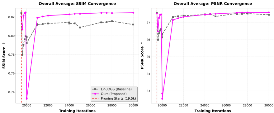
Figure 1: Training convergence. PSNR (dB) and SSIM after iteration 19,500 on Mip-NeRF 360. LinearMask-GS converges faster and to higher values than LP-3DGS.
