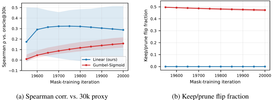
Figure 5: Ranking reliability on Mip-NeRF 360 across the mask-training window. (a) Spearman correlation between the mask ranking and the held-out max-pooled contribution proxy at 30k. (b) Fraction of keep/prune decisions flipped by re-sampling the Gumbel activation noise; the linear-increment mask is deterministic. Shaded regions show the min-max range over the nine scenes.
