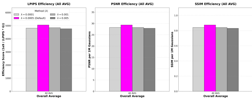
Figure 2: Sensitivity to \lambda_m . Efficiency score under varying \lambda_m on Mip-NeRF 360. The default \lambda_m = 5 \times 10^{-4} (highlighted) yields the best LPIPS-based efficiency score.
