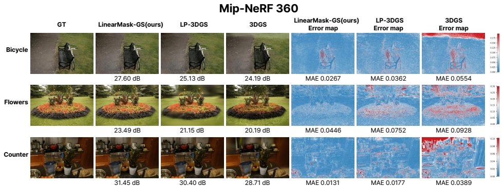
Figure 2: Per-scene qualitative comparison on three representative Mip-NeRF 360 scenes ( Bicycle , Flowers , Counter ). Each row: GT, renders from LinearMask-GS / LP-3DGS / 3DGS (PSNR below), then per-pixel absolute error maps for the same three (MAE below; scene-specific blue-to-red colormap). LinearMask-GS consistently shows lower error and fewer saturated red regions; remaining six scenes in the supplement.
