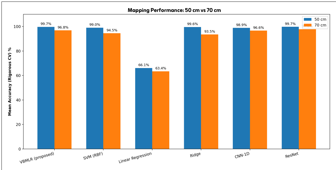
Figure 9: Mean zone accuracy (%) at 50 cm and 70 cm for all evaluated mappings under 5-fold stratified cross-validation.
