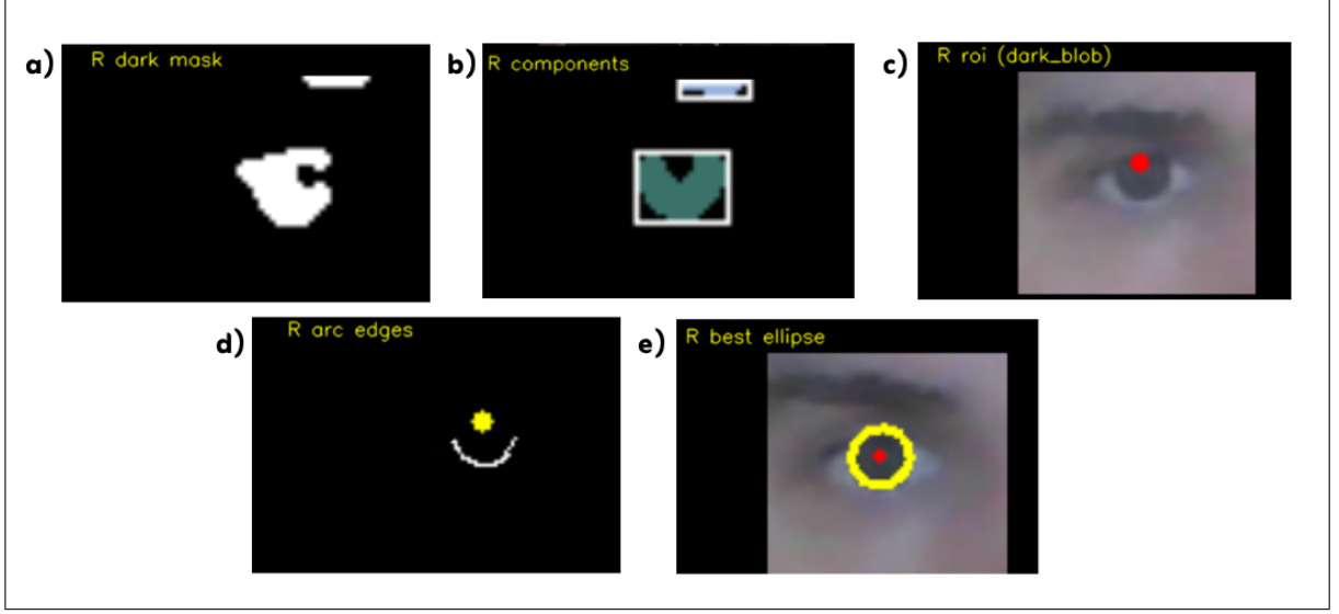
Figure 4: Main steps of iris-center estimation in the right eye. (a) Binary dark mask computed in the eye ROI. (b) Separate dark regions obtained from the mask. (c) Initial iris-center candidate obtained from the selected dark region. (d) Contour verification around the candidate center. (e) Refined iris-center measurement obtained from the fitted ellipse.
