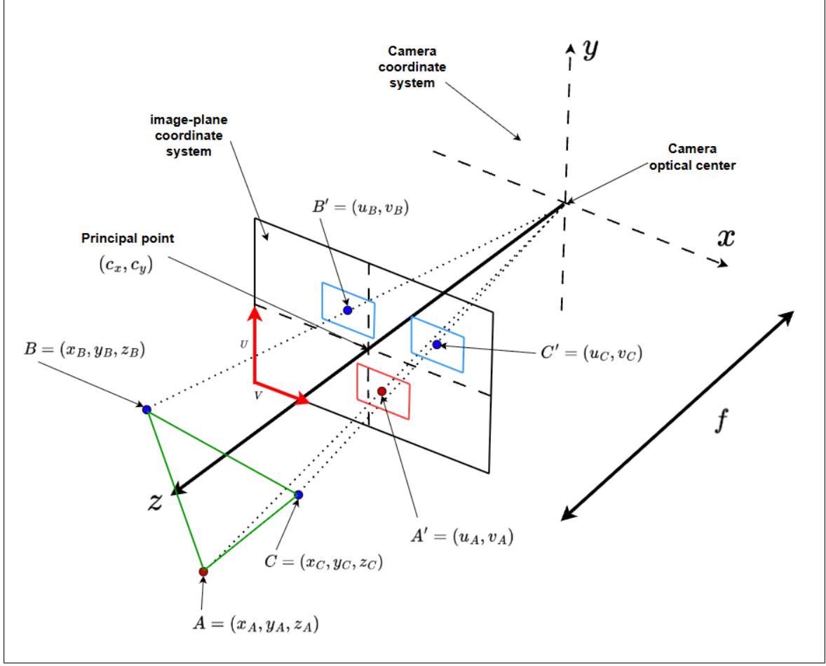
Figure 7: Geometry used for head pose estimation. The image points A' , B' , and C' are extracted from the detected facial regions and assigned depths z_A , z_B , and z_C estimated from blur. These depths are then used to calculate the 3D points A , B , and C .
