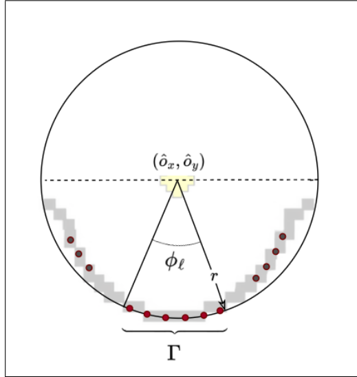
Figure 5: Circular-contour evaluation around the initial iris-center candidate (\hat{o}_x, \hat{o}_y) . The angle \phi_\ell defines a sampled direction and r denotes the tested radius. The retained directions \Gamma are represented by their intersections with the tested circular contour along the visible iris-contour portion.
