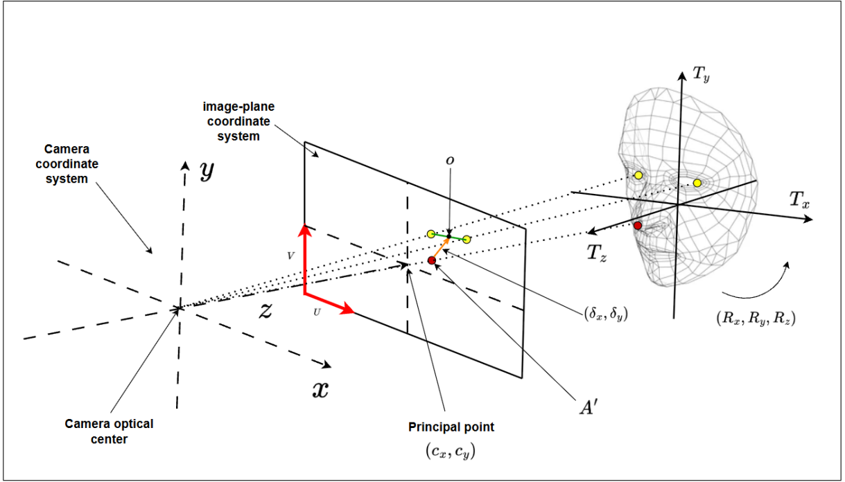
Figure 2: Representation of the coordinate systems and gaze parameters used in the proposed method. In the image-plane coordinate system, the iris displacement vector \delta = (\delta_x, \delta_y) is defined from the nose center A' to the mean iris position o . In the camera coordinate system, the head-position vector T = (T_x, T_y, T_z) and the head-orientation vector R = (R_x, R_y, R_z) describe the position and orientation of the head relative to the camera optical center.
