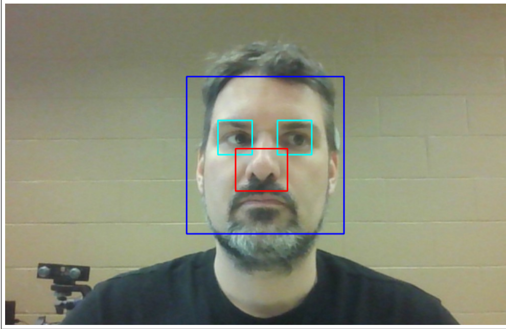
Figure 3: Example of the detected face region, the eye regions derived from the face bounding box, and the detected nose region.
