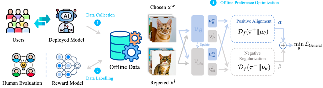
Figure 1: FLOWCPO uses a fixed preference dataset to train two coupled flow branches. A frozen generator supplies preferred/dispreferred pairs \mathcal{D} = \{(c, x_0^w, x_0^l)\} ; the positive branch matches preferred samples, while a mirrored branch matches dispreferred samples. Training uses only noised versions of these fixed endpoints and requires no online rollout.
