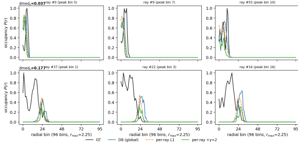
Figure 2: Example ray profiles for a mid- and a hard object. GT profiles (black) are narrow with peak \approx 1 ; D8 (blue) is over-wide and low; the per-ray model (orange) is sharper; the sharpened-target model (green, \gamma=2 ) matches GT width on covered rays. Three covered rays (peak bins at the 25/50/75 percentiles) are shown per object.
