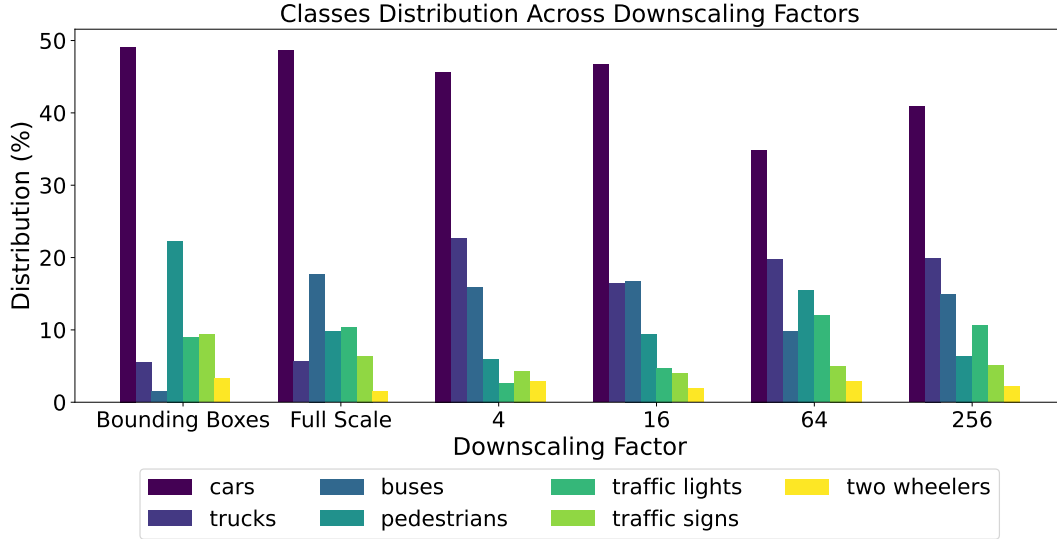
Figure 5: Distribution of ROIs per class across the various downscaling factors. Dataset bounding boxes values are on the left.
