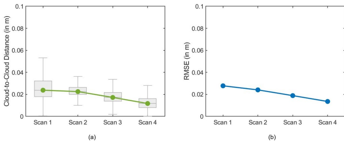
Figure 8. Accuracy assessment of the 3D-TARGeT georeferencing results across the four multi-temporal stope scans: (a) cloud-to-cloud (C2C) distance distributions and median C2C distances, and (b) corresponding C2C RMSE for each scan.
