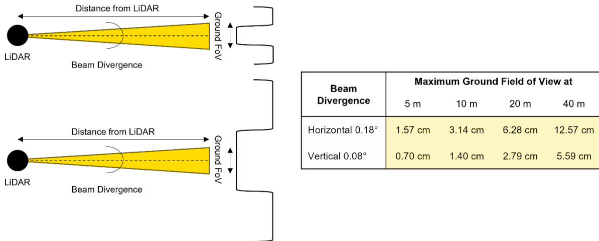
Figure 2. Effect of LiDAR static beam divergence on the resulting laser footprint at different scanning distances.
