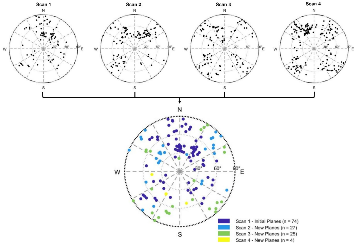
Figure 10. Time-series structure across the four georeferenced stope scans. Individual stereonet show the discontinuity orientations identified in each scan, while the combined stereonet presents the initial planes from Scan 1 and newly emerging planes in Scans 2-4.
