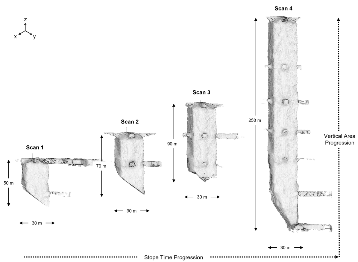
Figure 1. Multi-temporal progression of the study stope showing four representative point cloud scans acquired at different stages of excavation. The marked approximate dimensions illustrate the progressive increase in stope vertical extent, while maintaining an approximately constant plan width.
