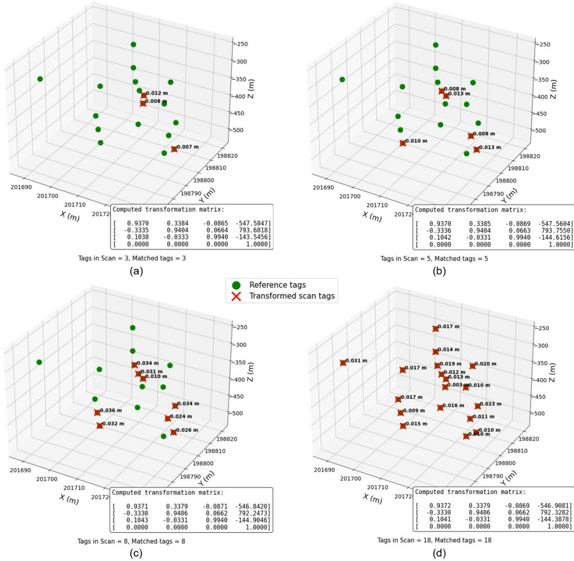
Figure 7. Tag-matching results leading to the refined registration and georeferencing of the four multi-temporal stope point clouds: (a) Scan 1, (b) Scan 2, (c) Scan 3, and (d) Scan 4, showing the refined centre and corner RMSE and the final transformation matrix for each scan.
