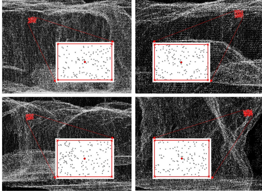
Figure 6. Identified candidate generic rectangular georeferencing tags within the stope point clouds, with enlarged views showing the identified tag points, with the reconstructed boundaries, centres, and four corners.
