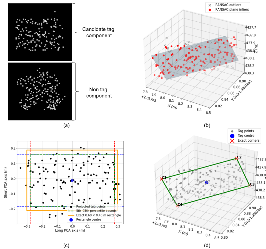
Figure 5. Sequential identification of the generic georeferencing tag using 3D-TARGeT: (a) representative components isolated by connected-component segmentation, including a candidate tag component with inherent noise and undefined edges and a non-tag component representing a random stray mine feature; (b) RANSAC segmentation of the candidate component showing the fitted plane, planar inliers, and rejected outliers; (c) PCA projection of the planar inliers with 5th–95th percentile edge estimation and reconstruction of the nominal 0.60 m × 0.40 m tag geometry; and (d) final identified tag showing the reconstructed rectangular boundary, estimated centre, and four corners used for subsequent registration and georeferencing.
