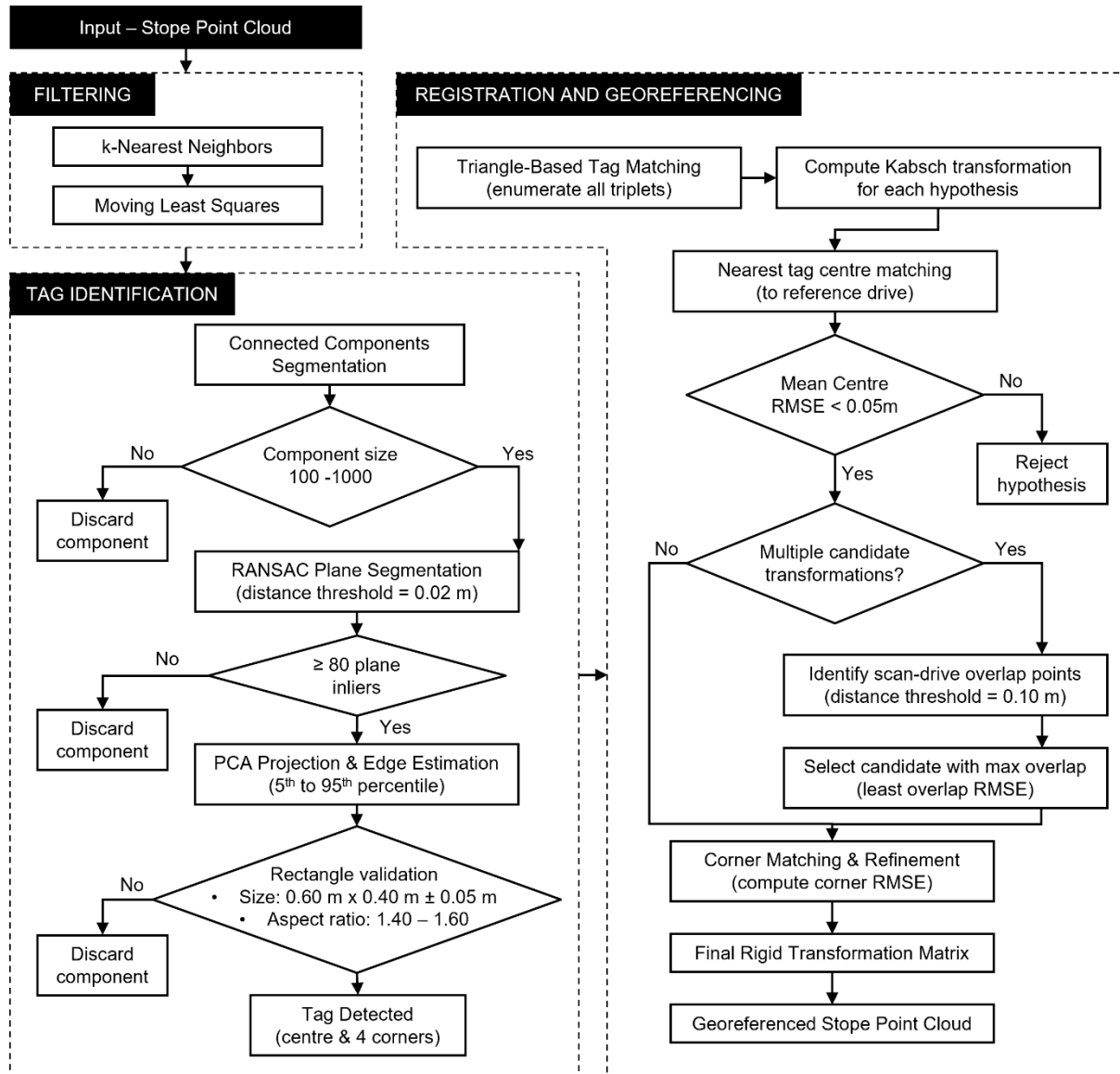
Figure 4. A detailed overview of the 3D-TARGeT algorithm used in this study.
