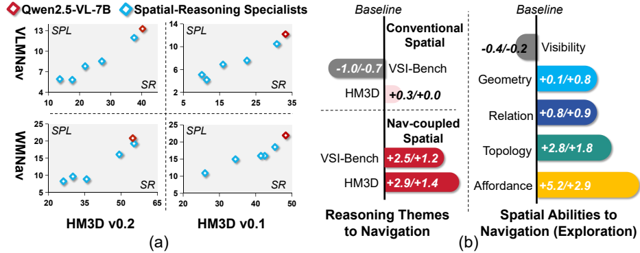
Figure 2: Summary of analysis about the relationship of spatial reasoning and navigation. Benchmark-oriented spatial specialization does not improve navigation (a). Spatial reasoning coupled to navigation goal gives consistent gains, and different spatial abilities help at different navigation phases (b).
