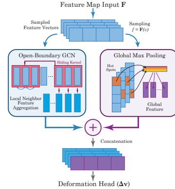
Fig. 3: Dual-Stream Architecture. Local (OBC) and Global feature streams fuse to guide deformation.
