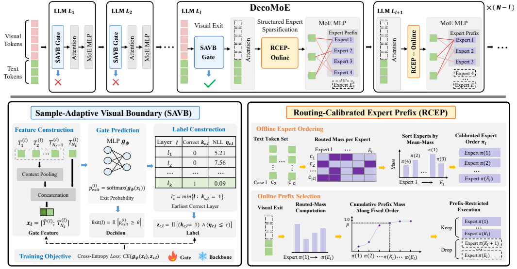
Figure 2: Overview of DecoMoE. Top : At each candidate-layer entrance, SAVB determines whether to remove the complete visual-token block before self-attention. Once triggered at layer l , RCEP is activated in the MoE block of the same layer and independently restricts the triggering layer and each subsequent MoE layer to a mass-sufficient contiguous prefix of offline-reordered experts. Bottom left : SAVB constructs its gate feature from the pooled preceding text states and the final text state, and is trained with labels derived from forced-exit correctness and first-token NLL while the backbone remains frozen. Bottom right : Offline, RCEP derives a layer-wise Mean-Mass expert order from cross-case text-token routing. Online, it aggregates the activated routed mass over tokens in each MoE invocation and retains the shortest prefix covering the target mass fraction p .
