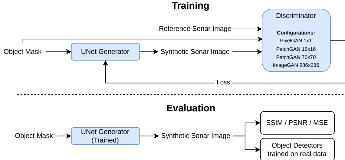
Fig. 2: Pix2Pix-based synthetic sonar generation and evaluation pipeline with different discriminator receptive fields
