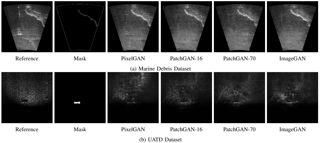
Fig. 3: Qualitative comparison of generated sonar images across discriminator configurations and datasets.
