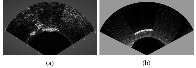
Fig. 1: Comparative Visualization of Sonar Data: (a) Real sonar image (b) Simulated sonar image [3].
