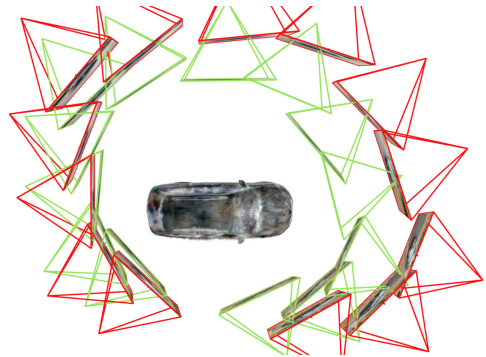
Fig. 14 Failure case: extreme-viewpoint extrapolation. The capture orbits the car at mid-height; rendered from directly overhead, far outside the observed viewing directions, the appearance breaks down, although the geometry stays on the CAD surface.
