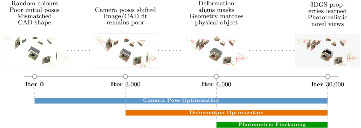
Fig. 5 Evolution of the CADSplat Optimization process. (Top) The visual state of the 3DGS representation at key iteration milestones. (Bottom) The active optimization parameters over the course of training.
