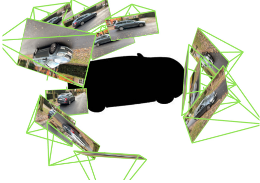
(b) Independent per-camera silhouette matching
