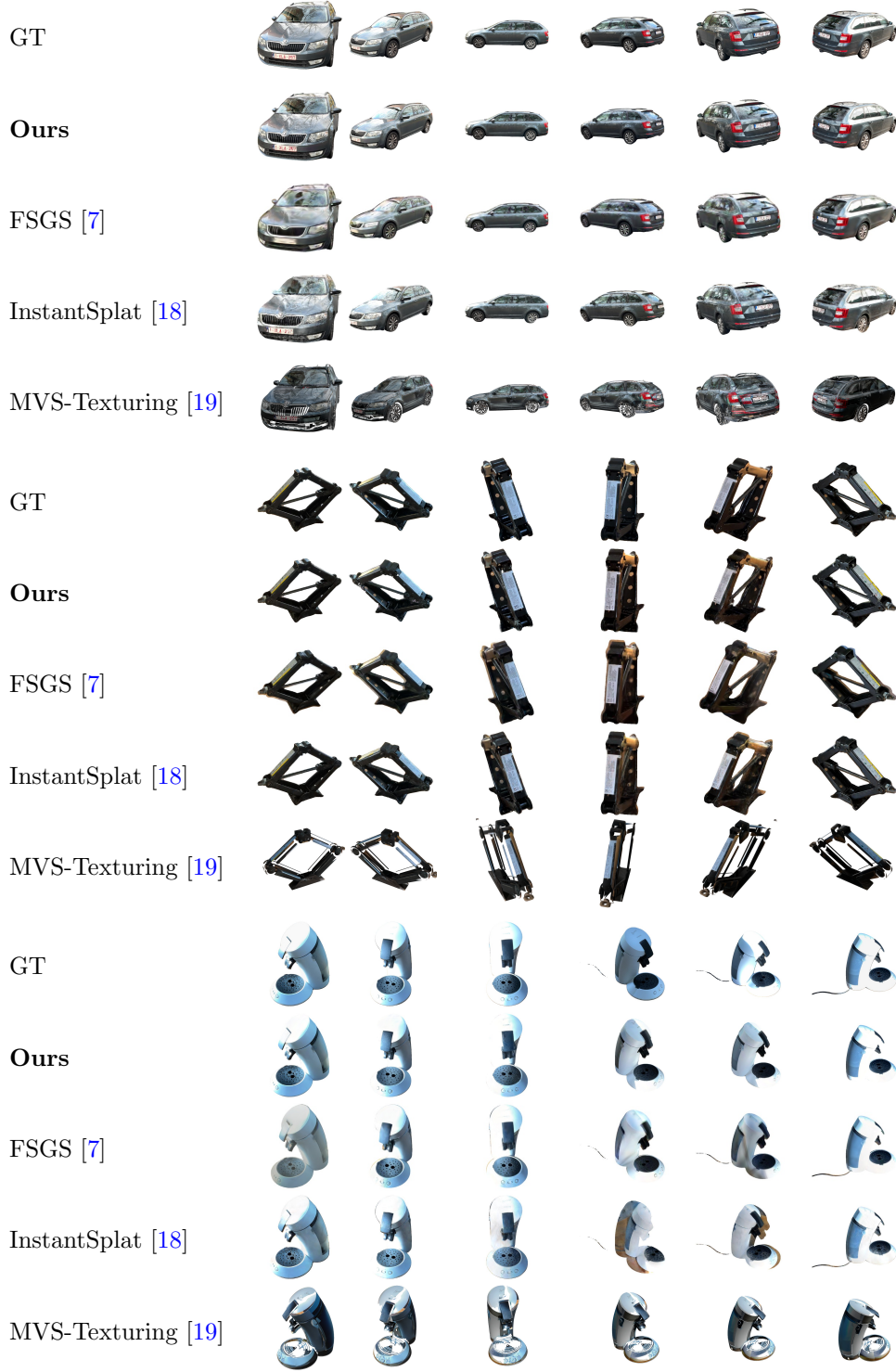
Fig. 7 Qualitative comparison on sparse-view reconstruction (9–13 images). MVS-Texturing [19] produces an inconsistent patchwork of textures and leaves weakly observed regions untextured. FSGS [7] suffers from over-smoothing. InstantSplat [18] is an SfM-free full-scene method; as it reconstructs the whole scene rather than the object, its tiles are shown composited with the ground-truth mask, and even then, it recovers only a coarse object with distorted geometry and smeared texture. CADSplat (Ours) maintains strict geometric fidelity, preserving sharp edges and accurate textures. Best viewed digitally and zoomed in.
