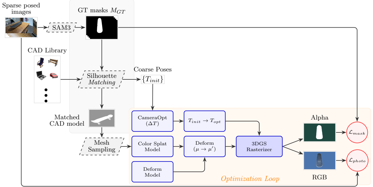
Fig. 2 CADSplat overview. Object silhouettes from SAM3 [43] are matched against renderings of a CAD library to retrieve the most similar model and coarse camera-to-object poses. 3D Gaussians are sampled on the retrieved mesh, and the deformation network, camera correction, and 3DGS parameters are then optimized jointly. During the geometric warmup, only the rendered alpha channel is supervised against the mask M_{GT} ( \mathcal{L}_{mask} ); afterward, the rendered RGB is compared with the masked photographs ( \mathcal{L}_{photo} ).
