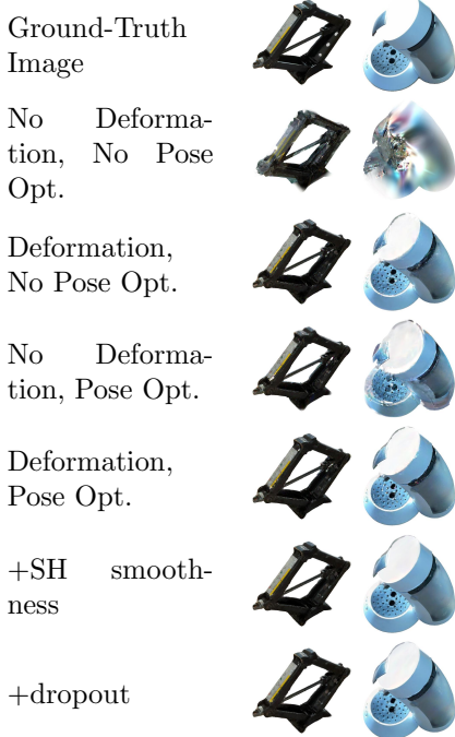
Fig. 9 Visual ablation study demonstrating the impact of architectural decisions on the reconstruction quality.
