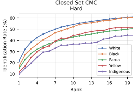
Fig. 7. Closed-set identification (1:N) performance of a single R50+ArcFace model by race/color group, shown as CMC curves on the hard set.
