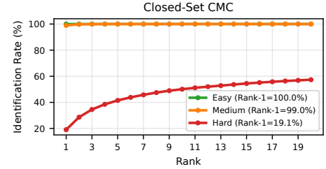
(b) Closed-set CMC by difficulty.
