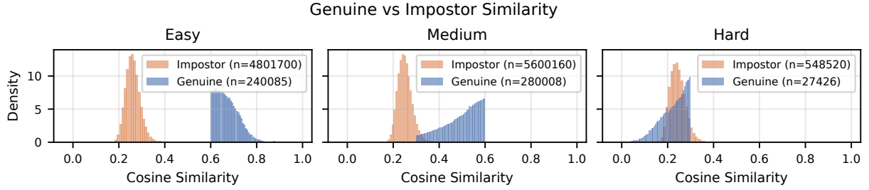
Fig. 4. Cosine similarities between impostor and genuine pairs in the three subsets: easy, medium, and hard.
