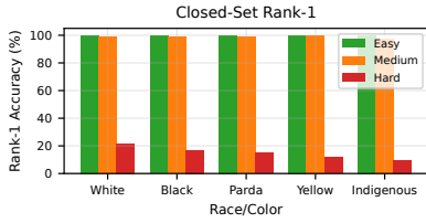
Fig. 6. Performance analysis of the model on the UFPR-PES benchmark. Closed-set rank-1 accuracy of the model by race/color and difficulty subset.
