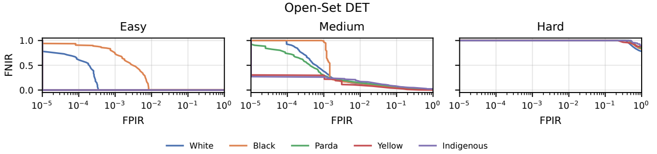
Fig. 8. Open-set identification analysis of the model R50+ArcFace by race/color and difficulty subsets on our UFPR-PES benchmark.
