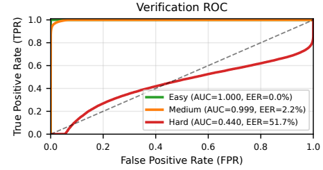
(a) Verification ROC by difficulty.
