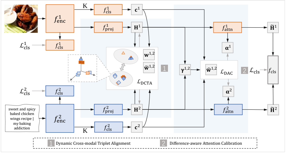
Figure 1: Overview of the proposed framework ACML. In \mathcal{L}_{DCTA} , \Delta and \square denote different categories, colors represent modalities, and color intensity reflects confidence.
