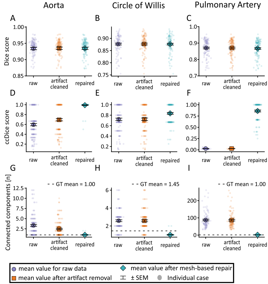
Fig. 4. Quantitative summary of repair effects and mesh-fitting convergence. Mesh-guided repair improves connectivity-oriented metrics while preserving Dice, and meta-initialization accelerates per-case mesh fitting.
