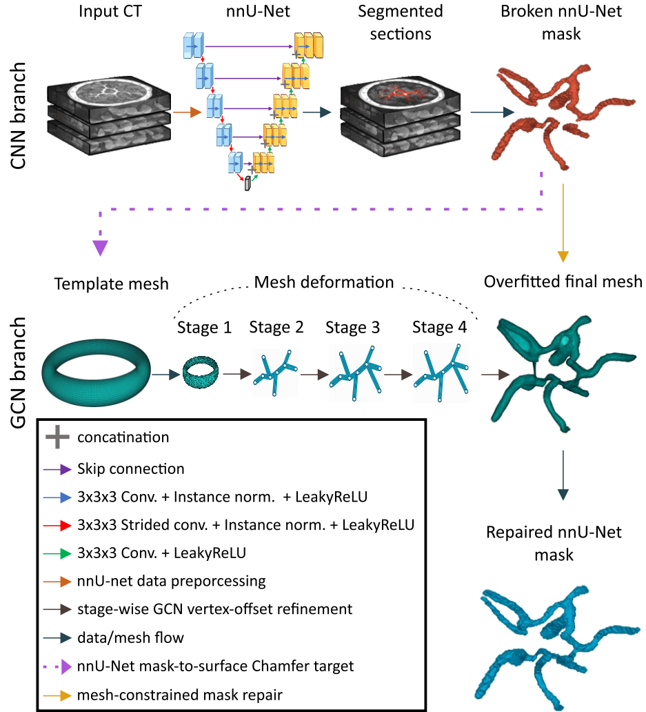
Fig. 2. Overview of the proposed mesh-guided nnU-Net repair pipeline. A CT volume is first processed by a CNN segmentation branch based on nnU-Net, producing segmented vessel sections and an initial nnU-Net mask. When the predicted mask is fragmented or topologically inconsistent, its surface is extracted and used as the target for mesh fitting. Then, a fixed template mesh is passed through a GCN deformation branch. The mesh is progressively refined over multiple deformation stages, where each stage predicts bounded vertex offsets and forwards the updated mesh to the next refinement stage. The final overfitted mesh approximates the surface geometry of the nnU-Net prediction while preserving the template mesh connectivity. This fitted mesh is then used as a geometric prior for topology-aware mask repair, producing a repaired nnU-Net mask with improved connectivity.
