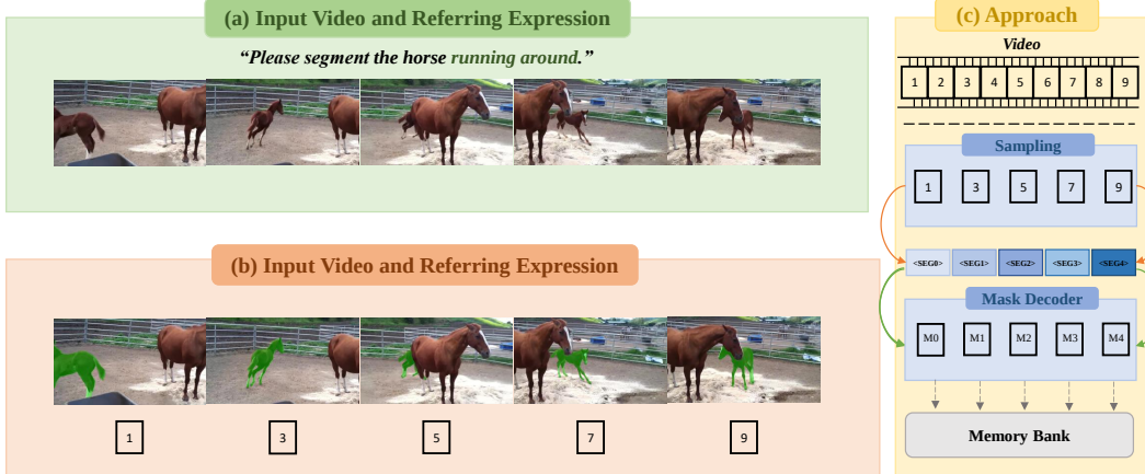
Figure 1: Overview of MoVISA. Given an input video and a referring expression, MoVISA samples a subset of key frames and generates one segmentation token per frame. The segmentation tokens are processed by a mask decoder to generate the corresponding masks, which are then added to a memory bank for mask propagation to non-key frames.
