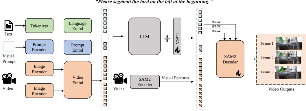
Figure 2: Overview of our network architecture. A Large Language Model (LLM) processes the input language and video embeddings and generates multiple segmentation tokens. These segmentation tokens are fed into the SAM2 mask decoder to generate the output segmentation.
