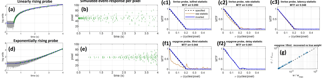
Fig. 3. Monotonically rising probes. (a) For a linear rising probe in log-irradiance values, we see continuously emitted events with ever increasing intervals. (b) For a full 1-D sensor simulated response to the input through h(x) the events per pixel are presented as green marks in relation to time. Measurement time and slope value was tuned to produce the overall same count of events as in Fig. 2 - with a maximal event count of 17 for the highest intensity step, and an overall count of 174 events over the 101 simulated pixels. Estimation of the specified MTF is shown using (c1) the first interval, (c2) mean rate, (c3) and first event latency, with error RMS roughly 5% for all those methods. For each, we present the inverse-function based estimation (blue line), and direct-from-event estimation (teal-line), compared to the specified ground truth (where teal-line not present, it is underneath the blue line, indicating no inverse is needed in practice). (d) Similarly, an exponentially rising input signal is analysed, (e) also tuned to have a similar event count across the array (17 events at peak pixel, and 172 event in total), and an MTF reconstruction error of (f1) 4.4% for first interval inverse, and (f2) 6.1% for first event delay. (g) Presenting the optical weight estimated from the first interval shows ideal match to the expected value for each pixel, indicating the MTF error is only attributed to discretisation error (sub-threshold pixels).
