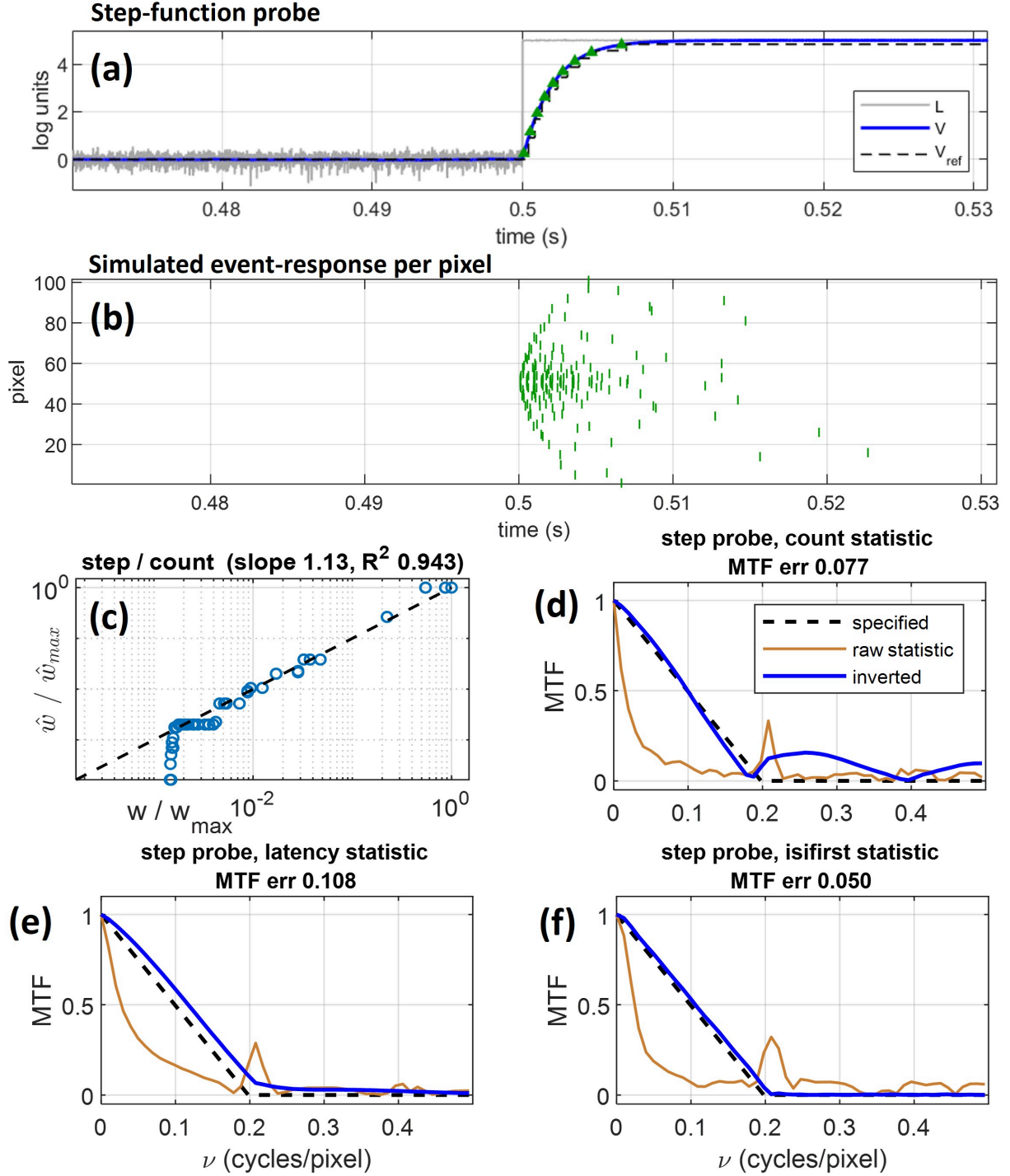
Fig. 2. A step probe. (a) The simulated log-irradiance of a pixel (gray line), its source-follower voltage (blue), and the emitted events (green triangles) with their corresponding reference voltage (dashed line) as responding to a step function increase of intensity from I_{bg} = 2.5 \cdot 10^6 photons/sec to I = 1.8 \cdot 10^9 photons/sec, and a contrast threshold of C = 0.25 log units. (b) For the full 1-D sensor response to the step, with a spatial intensity distribution profile as in Fig. 1(d), where events per pixel are presented as green marks - with a maximal event count of 9 for the highest intensity step, and an overall count of 173 events over the 101 simulated pixels. (c) The pixel-intensity weight estimation (normalised) from equation (25), compared to the ground truth pixel weights, and a dashed line to rks expected for ideal reconstruction. (d) The estimated MTF from the inverted event-count from equation (17) (blue line), compared to the non-inverted attempt to measure MTF from counts (brown line), and the specified ground-truth MTF (dashed line). Similarly, the non-inverted and inverted estimation of MTF are presented for (e) the latency from step onset, and (f) first ISI. Corresponding RMS error for the estimation across the entire band is 7.7%, 10.8%, and 5% for the count-based, first event latency, and first ISI respectively.
