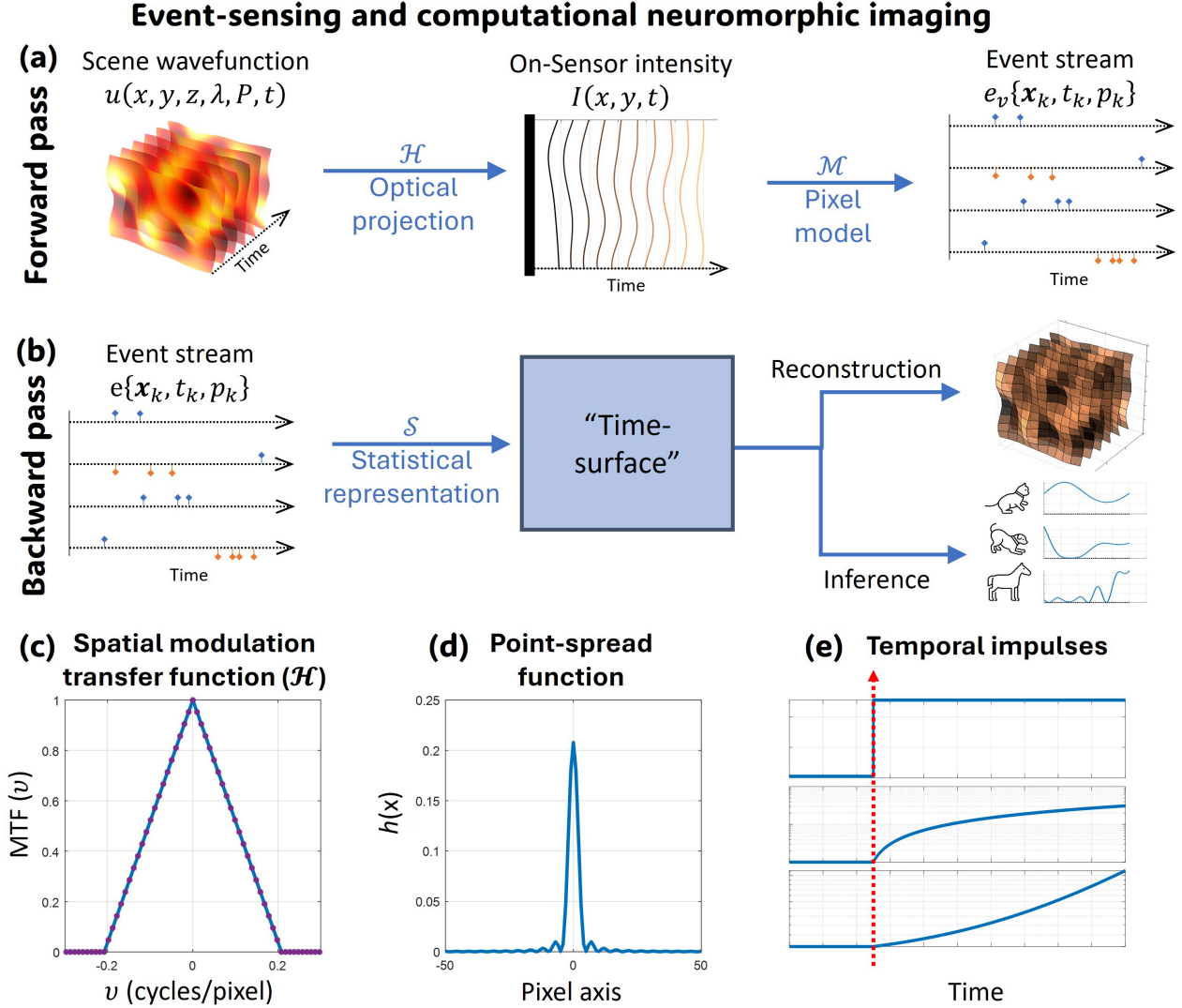
Fig. 1. Computational Neuromorphic Imaging framework, and the role of spatial-temporal probes in it. (a) A scene is projected through the optical components onto the Focal-Plane Array (FPA), and the corresponding spatial temporal signal is converted into an event-stream. This forward pass can be described by a spatial operation in the optics ( \mathcal{H} ) and a temporal point-process operator through the event-pixel model \mathcal{M} . (b) A backward pass must then disassociate these spatial and temporal operations by observing the statistics of the event-stream (often coined the “time-surface”), to successfully perform any inference or reconstruction task of the input scene. Useful tools to probe the relation between event-stream statistics and the spatial and temporal operations are the (c) MTF (related to the Optical Transfer Function (OTF)), (d) its corresponding PSF, and the (e) temporal impulse response. Shown here is an example of a trivial 1D rectangular pupil, giving a sinc-squared intensity PSF and a triangular MTF, and a selection of temporal impulses - a step function, a linear rise, and an exponent rise (all presented in log-intensity)
