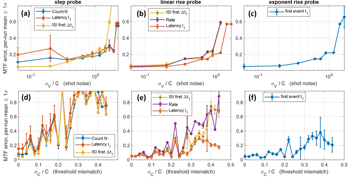
Fig. 4. Noise mode analysis for probes and their statistics. We consider the evolution of MTF estimation error with increased Poisson shot-noise for the (a) step function probe, (b) linear rise probe, and (c) exponential rise probe. The x-axis presents the standard deviation of the photon noise (estimated as the square root of the inverse photon flux), and normalised to the contrast ratio. For each we considered how the different statistical inverse chain performs, as detailed in Section III: event count N_i (blue line), first latency value l_{i,1} (red line), and first ISI \Delta t_{i,1} (yellow line) for step probe; first ISI \Delta t_{i,1} (yellow line), Rate R_i (purple line), and first latency value l_{i,1} (red line) for linear rise probe; first event time t_{i,1} for the exponential rise probe. Generally we see how the probes fail as the noise becomes equivalent to the contrast ratio ( \sigma_C/C \sim 1 ). Similarly, we consider how cross-pixel contrast threshold mismatch effects the MTF error, with (d) a step function probe analysis failing with any variation above 5%, while (e) a linear rise probe maintaining sub 20% accuracy even with 15% mismatch values, and the (f) exponential rise performing well even with around 20% normal mismatch.
