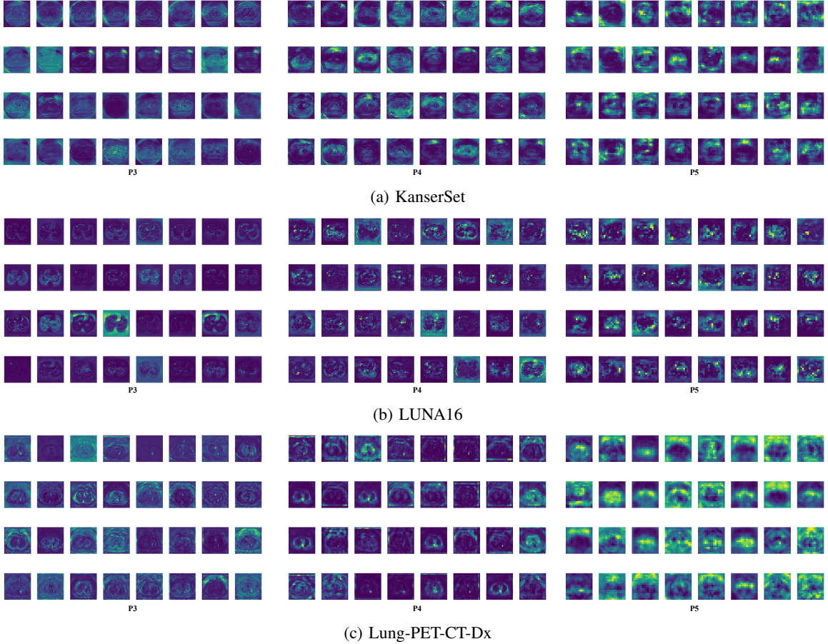
Fig. 7: Feature maps at P3, P4 and P5 across the three benchmarks, each row running from P3 on the left to P5 on the right. P3 shows radial boundary activation, P4 adds peri-nodular context with visible frequency separation, and P5 responds to broader anatomical neighborhoods. The same progression holds on every dataset.
