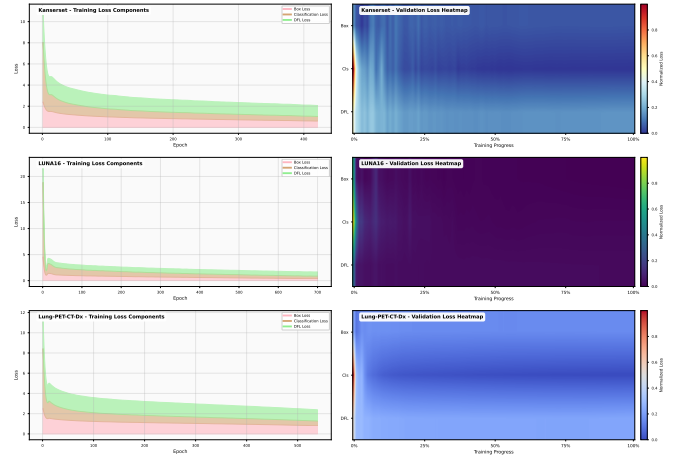
Fig. 5: Training and validation loss on the three datasets. Each left panel plots the box, classification and DFL training losses against epoch, and each right panel is a normalized validation-loss heatmap of the same components over training progress.
