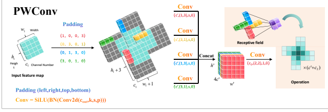
Fig. 3: PWConv. Four asymmetric branches with directional padding capture orthogonal gradient components through 1 \times 3 and 3 \times 1 kernels, followed by 2 \times 2 refinement.
