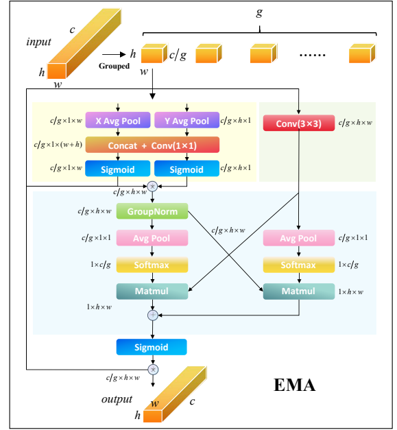
Fig. 4: Efficient Multi-scale Attention head. Features are split into eight groups and reweighted by parallel spatial and convolutional pathways with softmax-normalized cross-pathway gating.
