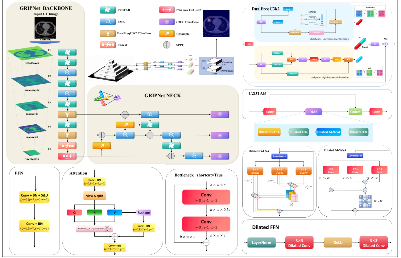
Fig. 2: GRIPNet architecture. PWConv replaces symmetric downsampling to capture radial gradients. DualFreqC3k2 at P4 and P5 splits features into high-frequency morphology and low-frequency context. C2DTAB fuses scales with dilated masked attention matched to the Gaussian decay range. EMA-enhanced heads at P3 to P5 give scale-adaptive prediction.
