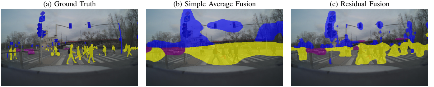
Fig. 5: Visual comparison of fusion strategies using CLFTv2-Tiny on ZOD. (a) Ground truth mask. (b) Simple averaging of RGB and LiDAR creates poorly defined boundaries. (c) Residual fusion recovers boundaries and suppresses structural artifacts.
