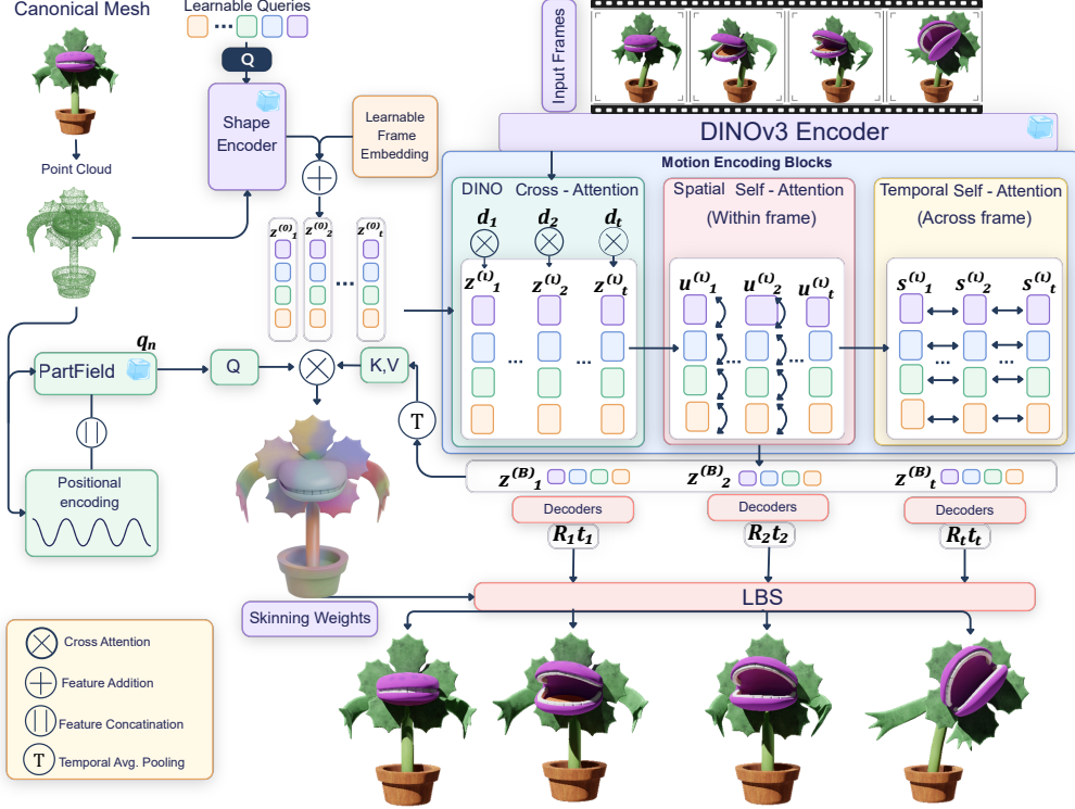
Figure 1: Method overview. BLARM takes a canonical mesh and a monocular video as input and represents the animation using a compact set of latent rigid motion components. Geometry-aware latents are conditioned on frame-wise DINOv3 features to predict time-varying rigid transformations, while time-invariant vertex-to-component skinning weights are learned without explicit skinning supervision . The final animated sequence is obtained by blending the predicted transformations through linear blend skinning.
