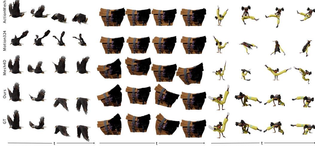
Figure 2: Qualitative comparison on ActionBench. Across diverse shapes, BLARM preserves the canonical mesh structure better than baselines and yields temporally more coherent animations with fewer jittering or distorted parts.
