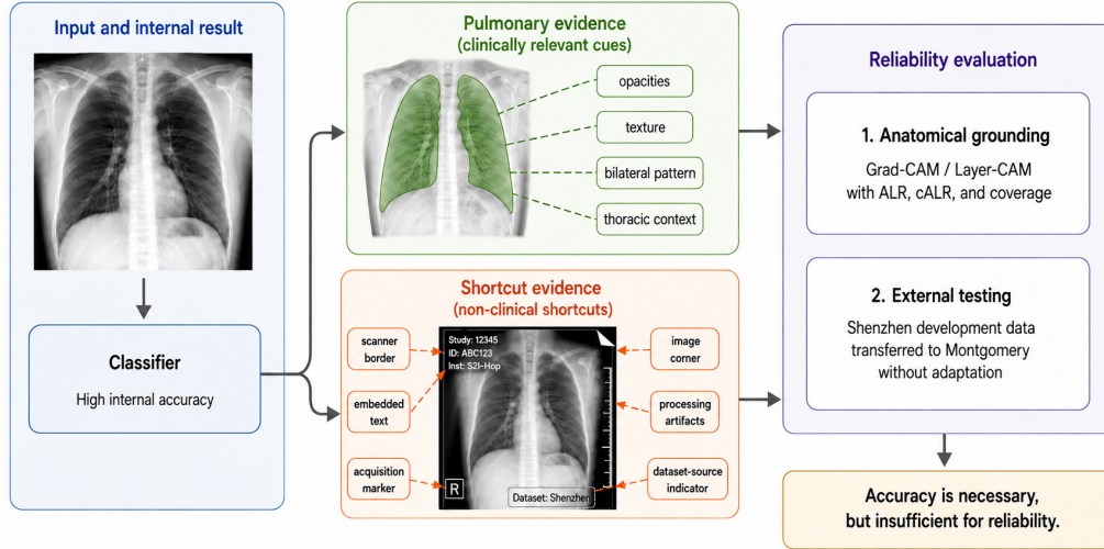
Figure 1: Reliability gap in chest X-ray classification: diagnostic performance versus pulmonary attribution containment and external robustness. Strong internal diagnostic performance does not establish whether class-related attribution is concentrated within the pulmonary field or whether diagnostic behavior is preserved under external cohort shift. The pulmonary anatomical prior represents the target anatomical region used for anatomy-guided feature aggregation. Potential non-pulmonary cues are shown as conceptual examples and are not presented as confirmed shortcuts used by the trained models.
