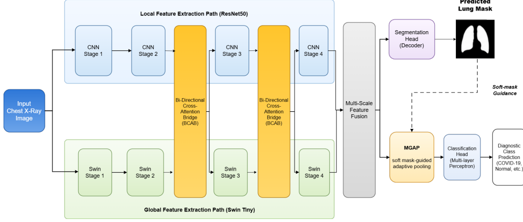
Figure 3: Overall DBCA-SegNet-MGAP architecture. The dual-encoder framework uses BCAB1 at 28 \times 28 , BCAB2 at 14 \times 14 , and final 7 \times 7 multi-scale feature fusion before pulmonary segmentation and mask-guided classification.
