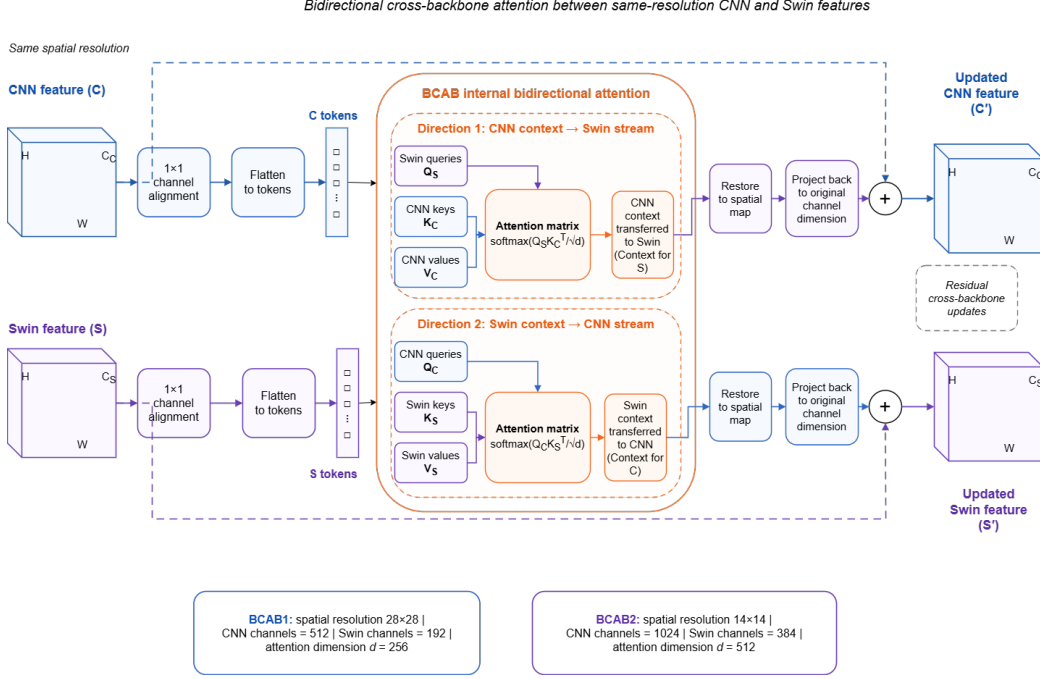
Figure 4: Internal mechanism of the Bidirectional Cross-Backbone Attention Block (BCAB). CNN context is transferred to the Swin stream, and Swin context is transferred to the CNN stream through reciprocal cross-attention and residual feature updates.
