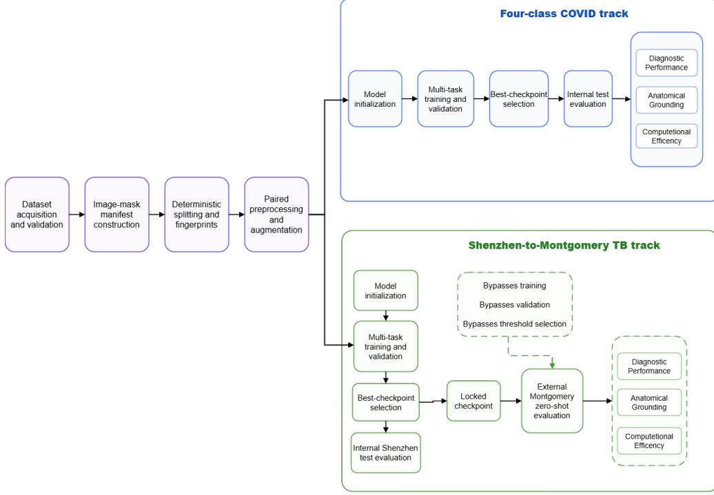
Figure 2: Experimental workflow for four-class COVID-19 evaluation and locked Shenzhen-to-Montgomery TB transfer. The COVID-19 track uses held-out internal testing, whereas the TB track uses Shenzhen for development and checkpoint selection followed by locked Montgomery zero-shot testing. Montgomery is not used for target-domain fine-tuning, recalibration, checkpoint reselection, or threshold optimization.
