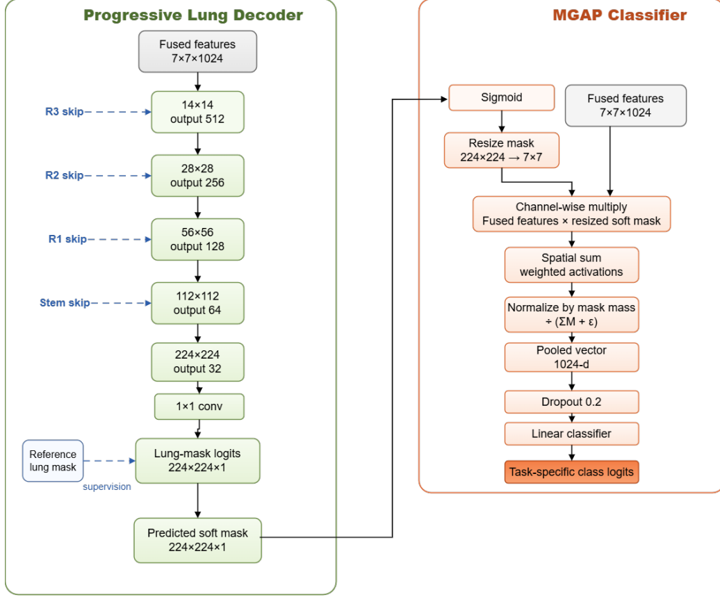
Figure 5: Progressive lung decoder and Mask-Guided Adaptive Global Average Pooling (MGAP) classifier. The decoder reconstructs a soft pulmonary mask from fused features and multiscale ResNet skip connections; MGAP resizes this mask to classifier resolution and uses it to weight normalized spatial feature aggregation.
