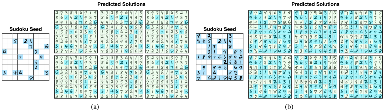
Figure 7: Output diversity of the Sudoku codec. (a) For an underconstrained clue pattern with at least 10^6 valid completions, repeated stochastic NCA rollouts produce multiple distinct valid solutions. (b) For a puzzle with a unique solution, resampling the decoder style latent preserves the solved board while varying the digit style.
