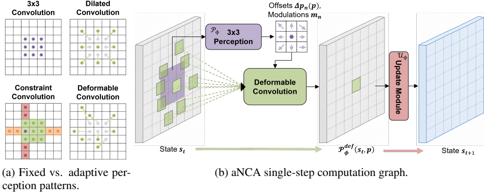
Figure 5: (a) Comparison of perception sampling patterns: standard 3 \times 3 , dilated, constraint-aligned, and deformable convolution. (b) One aNCA update step: the perception module \mathcal{P}_\phi predicts offsets \Delta \mathbf{p}_n(\mathbf{p}) and modulations m_n from s_t , which guide the deformable convolution to aggregate features from adaptive grid locations. The update module \mathcal{U}_\phi then produces the next state s_{t+1} .
