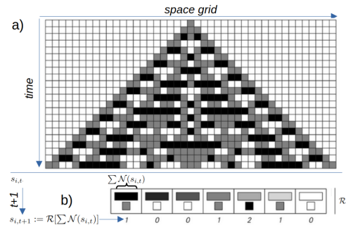
Figure 1: Sketch of a basic 1D Cellular Automaton with three discrete states s_i \in \{0, 1, 2\} and seven update rules \mathcal{R} . a) shows the inference of complex patterns from an initial state by the rules visualized in b) over time.
