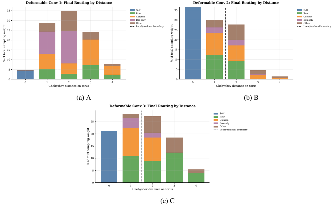
Figure 9: Learned sampling distance distributions of the three deformable perception heads (A, B, C) at the final NCA step, aggregated over held-out test puzzles. Each plot shows how far each kernel tap reaches from the source cell, revealing that the heads develop complementary routing strategies: some taps remain local while others extend to capture row, column, or box constraints.
