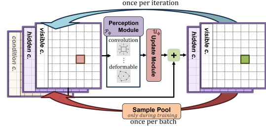
Figure 2: Sketch of a basic CNN implementation [34] of a 2D NCA with a 3D state space. The perception module processes the cell state using one of several configurable perception options. The update module processes the perceived features to compute state updates. Stochastic updates are applied before updating the visible and hidden channels to form the new cell state for the next iteration. The sample pool is used after one batch of images is processed to retain and reuse evolved states for subsequent training iterations.
