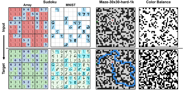
Figure 3: The four 2D spatial reasoning tasks evaluated in this work. Each column shows the input (top) and target (bottom).
