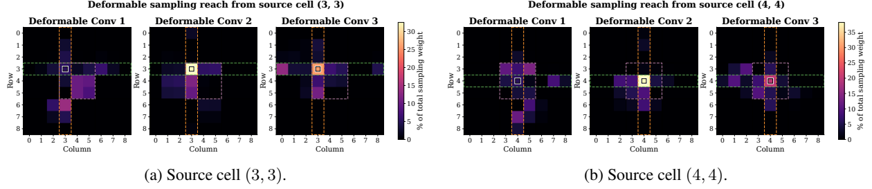
Figure 6: Learned sampling reach of each deformable perception head from two interior source cells (black-bordered squares at grid positions (3,3) and (4,4)). Each panel is one head: the heatmap shows the fraction of the head’s total sampling weight placed on every cell of the 9 \times 9 board, aggregated over held-out test puzzles at the final NCA step. Dashed overlays mark the source cell’s row (green), column (orange), and 3 \times 3 box (purple). The learned heat concentrates inside these overlays and the three heads specialize to complementary constraint directions.
