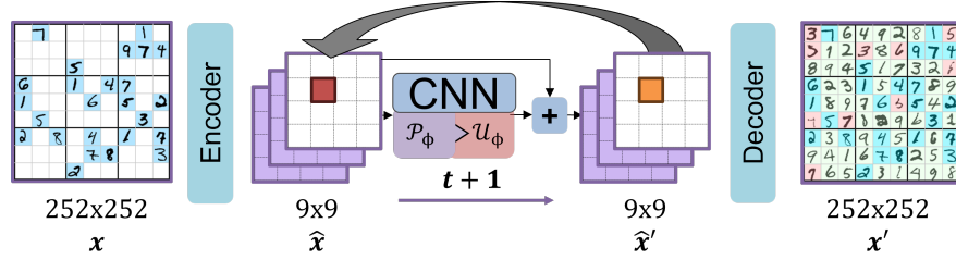
Figure 4: Latent pixel Sudoku pipeline. The encoder E_\psi maps the initial handwritten Sudoku image into a 9 \times 9 \times 9 grid of digit logits, the NCA iterates in this latent board space under the Sudoku constraint loss until a valid completion emerges, and the decoder D_\omega renders the final board back to pixels. Freezing E_\psi and D_\omega decouples perception from reasoning and allows different NCA variants to be evaluated within the same image-space pipeline.
