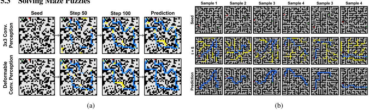
Figure 8: (a) Maze solving: the model receives walls (black), start (green), and goal (red). Blue cells indicate correct path predictions matching the target; yellow cells are predicted path pixels that deviate from the target. (b) Generalization to unseen 30 \times 30 Prim-style maze structures.
