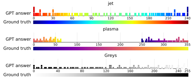
Figure 5: Innate Colormap produced by MLLM vs. the ground truth colormap used in our experiment. Observations. MLLM flipped some values along the map, which caused the negative \alpha values in the Stevens’s power law modeling.
