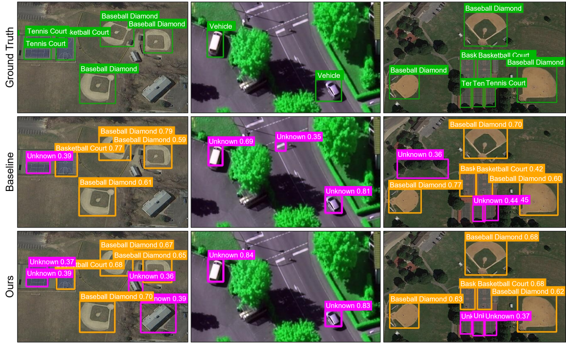
Fig. 4. Qualitative comparison on the NWPU VHR-10 dataset. The first row shows the ground-truth annotations (green), while the second and third rows show the predictions of the baseline and our method, respectively. Orange and magenta boxes denote known and unknown objects, respectively.
