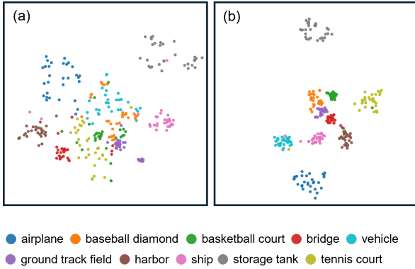
Fig. 6. The t-SNE visualization of proposal embeddings learned without (a) and with (b) the HML module.
