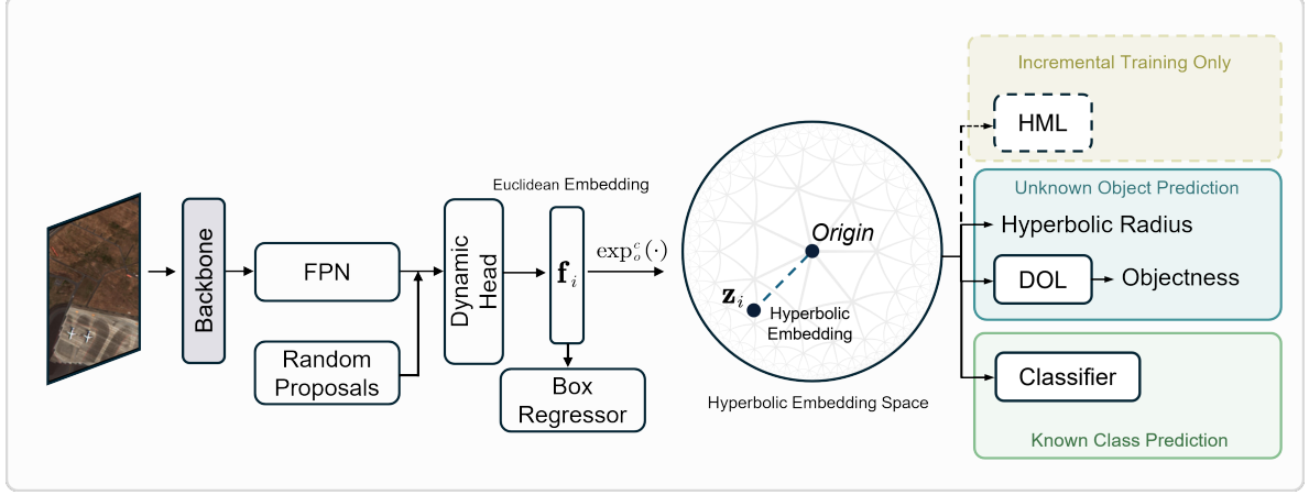
Fig. 2. Overview of our proposed HyRS-OWOD framework. The backbone and FPN extract multi-scale features from an input image, which are processed together with randomly generated proposals by the dynamic head to obtain proposal features \mathbf{f}_i . These features are used for bounding-box regression and mapped into the Poincaré ball via the exponential map \exp_0^c(\cdot) . For unknown-object prediction, DOL estimates class-agnostic objectness, while HUL measures uncertainty using the hyperbolic radius; proposals with high objectness and high hyperbolic uncertainty are identified as unknown. In parallel, the classifier predicts known object categories. During incremental training, HML is additionally applied to learn discriminative representations and mitigate catastrophic forgetting.
