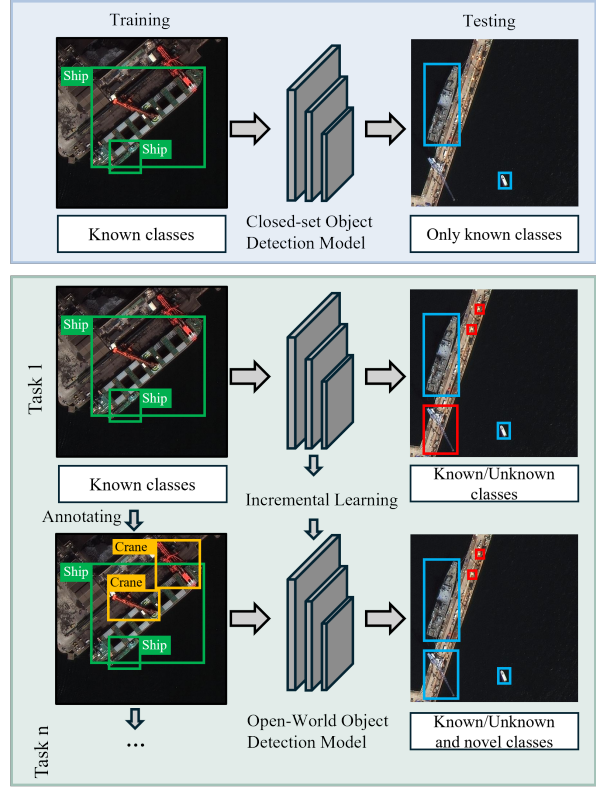
Fig. 1. Comparison between closed-set and open-world object detection in remote sensing imagery. Closed-set detectors recognize objects from only a predefined set of known categories, whereas OWOD additionally identifies unseen objects as unknown and incrementally learns them as novel classes once annotations become available.
