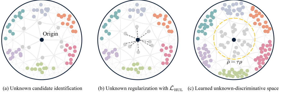
Fig. 3. Illustration of the proposed HUL strategy for known-unknown discrimination. Different colors represent proposals from different known classes, gray points denote candidate unknown proposals. (a) Candidate unknown proposals are selected for uncertainty-aware learning. (b) The HUL loss \mathcal{L}_{\text{HUL}} encourages candidate unknown proposals to lie in the high-uncertainty region near the origin. (c) After training, uncertain unknown proposals tend to lie closer to the origin than confident known proposals. The yellow dashed circle represents the normalized radius threshold \tilde{\rho} = \tau_\rho used for known-unknown discrimination.
