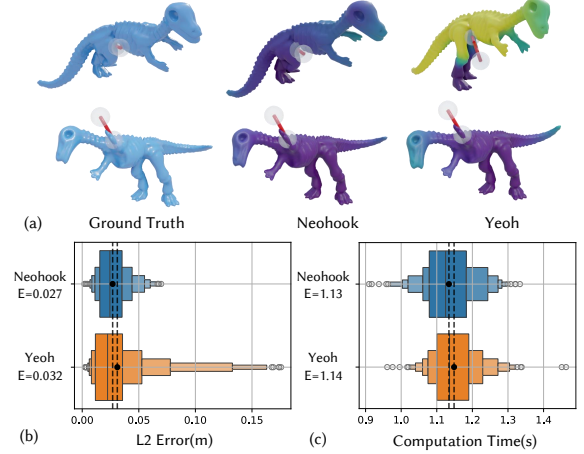
Fig. 12. Comparison of different material models tested with our pipeline. (a) Qualitative comparison between the ground-truth geometry and the adapted simulation results using the two material models. (b, c) With the proposed method, the Yeoh model shows similar computation time but less robust real-to-sim adaptation under large deformation.
