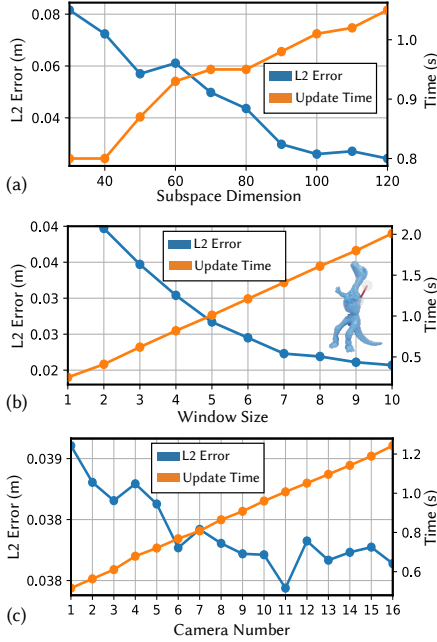
Fig. 11. Ablation studies on the Dinosaur model with random interactions. (a) Increasing the subspace dimension reduces the L2 error but increases the update time. (b) A larger temporal window size generally improves accuracy at the cost of longer update time (for this test, a fixed r = 100 is used). (c) Ablation on the number of camera views c for both reconstruction error and computational cost.
