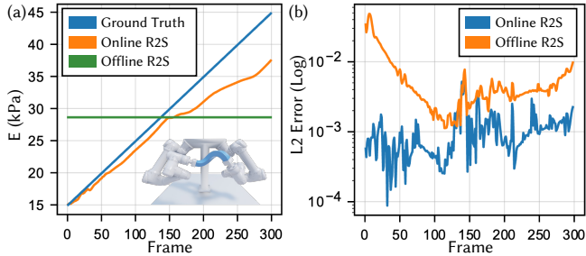
Fig. 9. Result and analysis of material aging in the bar manipulation task. (a) Our online real-to-sim method accurately tracks the time-varying Young’s modulus of the bar, whereas the offline baseline estimates an almost constant stiffness. (b) The per-frame L2 error further shows that online real-to-sim consistently outperforms the offline method.
