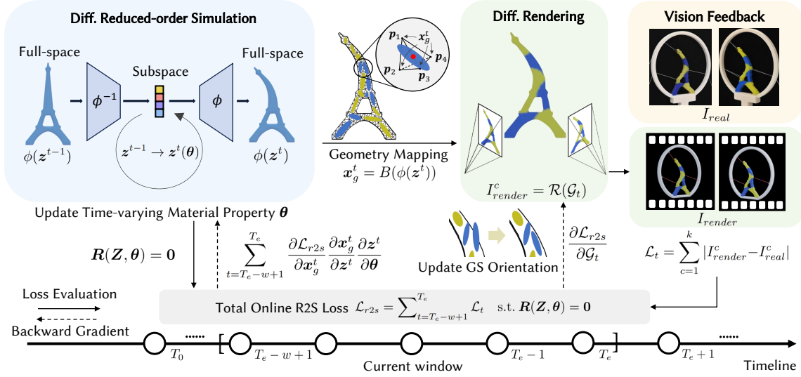
Fig. 2. Pipeline for online real-to-sim adaptation with vision-based feedback (i.e., sparse-view images I_{real} obtained from cameras). The forward process simulates deformation using a reduced-order model, maps the geometry to 3D Gaussians, and renders the image I_{render} through differentiable rendering to evaluate \mathcal{L}_{r2s} by updating time-varying material properties. The backward process back-propagates loss gradients to update material properties \theta and Gaussian orientations within a sliding window (i.e., from T_e-w+1 to T_e ), supporting gradient-based optimization to efficiently eliminate the real-sim difference.
