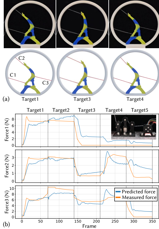
Fig. 5. (a) Additional real-to-sim adaptation result for cable-driven interaction with the multi-material Eiffel Tower model. (b) With the help of simulation, we can predict the cable force based on stress field reconstruction, which matches the ground-truth data captured by the force sensor, as shown in the zoom-in view.
