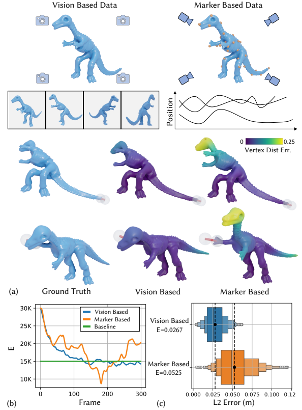
Fig. 10. Comparison of online real-to-sim adaptation on the dinosaur example using vision-based and marker-based physical input. 40 markers uniformly distributed are used for comparison. (a) Key frame showcase vision-based method outperforms in terms of reconstructed geometry accuracy. (b) Material parameter update curves during online adaptation. (c) Distribution of L2 errors over all frames for the two methods.
