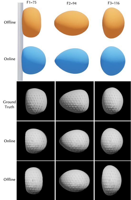
Fig. 7. Result of a high-speed ball bouncing back after hitting a wall with v_0 = 27\text{m/s} . The vision data are duplicated from IPC [Li et al. 2020], and the texture of the result is obtained by GS-based training.
