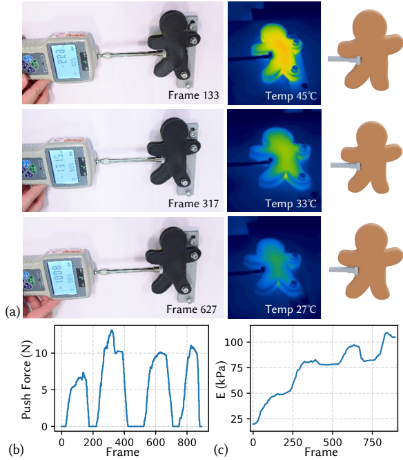
Fig. 6. Online real-to-sim adaptation for stiffness tracking in a temperature-varying structure. (a) Representative frames showing simulated deformation during cooling. (b) Push force over time. (c) Estimated Young’s modulus over time, demonstrating tracking of temperature-dependent stiffness variation.
