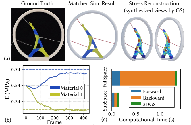
Fig. 3. Online real-to-sim results for a multi-material cable-driven deformable structure. (a) With vision feedback, the simulation results match the ground truth, enabling downstream applications such as stress reconstruction. (b) Convergence curves for the Young’s modulus of two silicone rubber materials. (c) Comparison with computation time showcases that our subspace solution achieves a 7.56 \times speedup, ensuring online efficiency.
