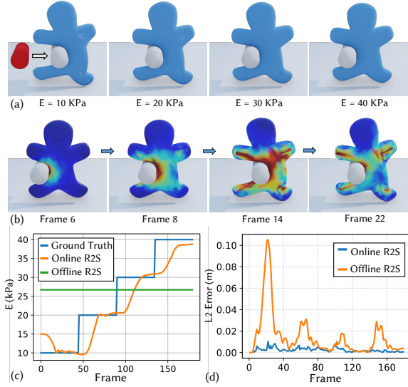
Fig. 8. (a) Comparison of deformation dynamics across different stiffness levels (Young’s modulus changing dynamically from 10 kPa to 40 kPa in steps when the bar is hit by the Gingerbread-man). (b) Reconstructed stress fields over time ( E = 10 kPa for all frames). (c) Prediction of time-varying Young’s modulus changes and (d) comparison of online and offline methods, showing that the proposed online framework tracks evolving stiffness.
