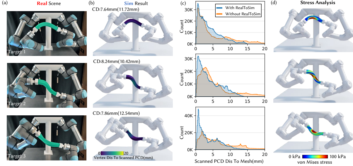
Fig. 4. Result for soft bar manipulation by dual robot arms. (a) After performing online real-to-sim adaptation, the control strategy optimized in simulation is directly applied to the real robotic system without additional tuning. (b) Corresponding simulation results after adaptation, colored by the vertex-to-scan distance. (c) Quantitative comparison between the simulated mesh and the ground-truth point cloud captured by a 3D scanner, demonstrating reduced geometric discrepancy after real-to-sim adaptation. (d) The adapted simulation with vision-based feedback further enables downstream physical analysis of von Mises stress reconstruction.
