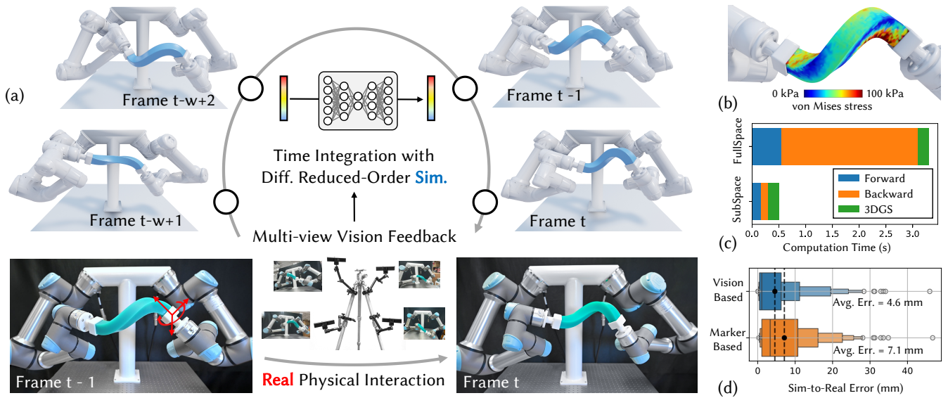
Fig. 1. We propose an online Real-to-Sim method to reduce the reality gap for deformable object manipulation. (a) In our pipeline, real-to-sim gap is eliminated by minimizing the difference between physical vision feedback and simulation-based rendered images within a sliding time window \{t - w + 1, \dots, t\} . In this way, we close the sim-real loop by integrating scene representation with 3D-GS, (b) and realize downstream applications like physical stress construction in arbitrary new synthesized views. (c) Neural reduced-order differentiable simulation is adopted, which significantly accelerates computation and achieves quasi-real-time performance, delivering 6.23x speedup over full-space methods. (d) Our method generalizes to physical inputs from conventional marker-based motion capture systems, whereas the vision-based solution performs better.
