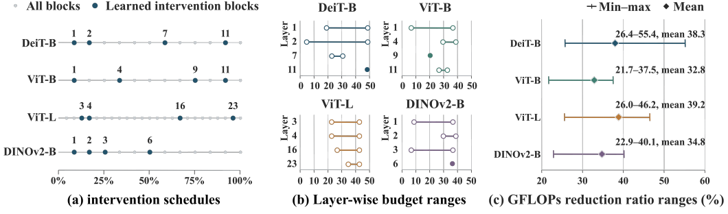
Figure 3: Learned adaptivity in where and how much to prune. (a) Intervention locations learned for each backbone. (b) Min-max deletion budgets over gate-active validation images at each intervention block; filled points denote collapsed single-budget decisions. (c) The resulting per-image GFLOPs-reduction ranges and means.
