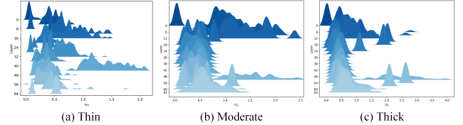
Figure 5: Layer-wise distributions of frozen channel-wise thresholds v_{th} learned on (a) thin, (b) moderate, and (c) thick haze subsets (dark-to-light: shallow-to-deep layers).
