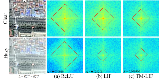
Figure 3: Frequency-domain visualizations under different neurons. The left shows clear and hazy remote sensing images with the region of interest highlighted, while the right compares ReLU, LIF, and TM-LIF in terms of spectra. We report \Delta , the high-frequency energy ratio drop from clear to hazy, which indicates that haze suppresses high-frequency components. Compared with LIF, TM-LIF, via channel-wise adaptive thresholds and multi-level quantization, yields spectra closer to the continuous responses of ReLU and alleviates the haze-induced loss of high-frequency details.
