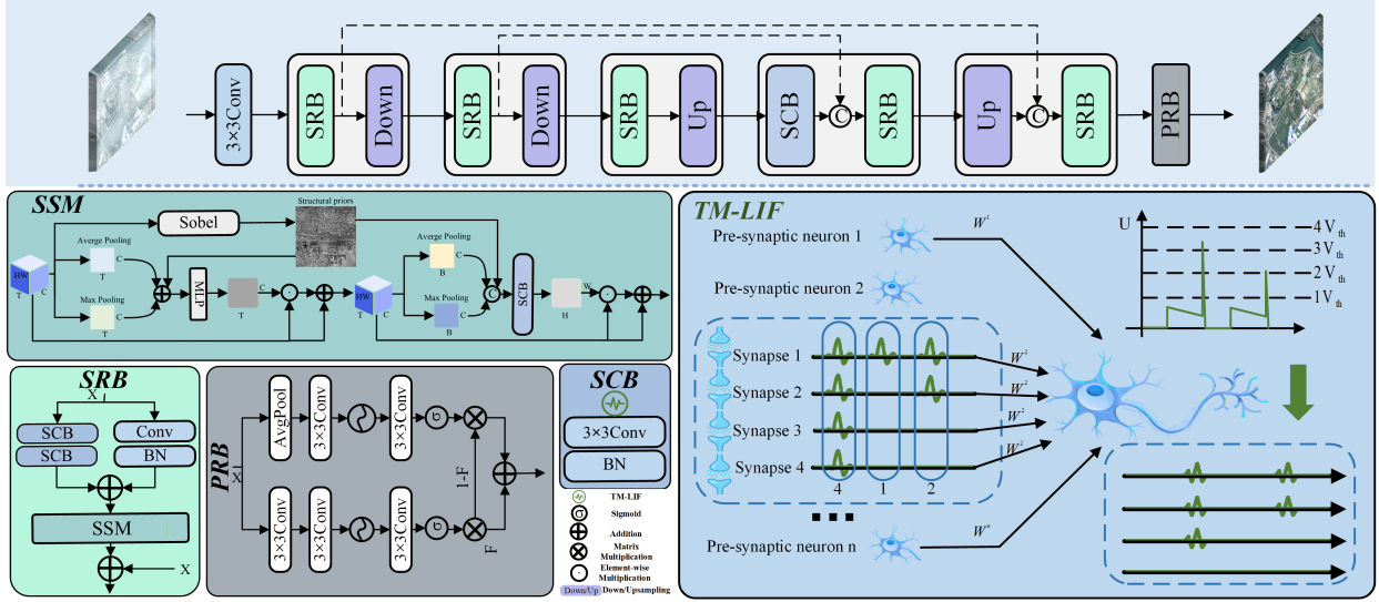
Figure 2: Overall architecture of EM-SNN. EM-SNN adopts a multi-scale encoder–decoder built from SRB blocks with skip fusion via channel-wise concatenation (C), and uses PRB for reconstruction. TM-LIF is applied in all SCB units across both SRB blocks and the Down/Upsampling stages, while SSM is embedded across scales to provide structure-guided attention.
