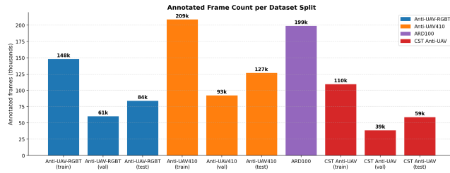
Figure 7: Per-split counts of UAV-present frames—frames in which a UAV is present (the exist=1 flag), labelled ‘annotated’ on the figure axis. Anti-UAV410 is the largest (428,703 across train/val/test), followed by Anti-UAV-RGBT (293,209). CST Anti-UAV (208,221) and ARD100 (199,291) are comparable in size; ARD100 is used only for motion-mask pre-computation and is not part of the continual learning curriculum.
