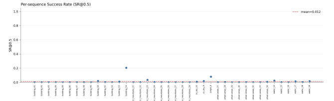
Figure 11: Per-sequence success rate at IoU 0.5 (SR@0.5) on CST Anti-UAV validation set. Sequences with predominantly tiny targets ( <256 \text{ px}^2 ) show the lowest SR@0.5, consistent with the near-zero tiny-stratum mAP reported in Table 1.
