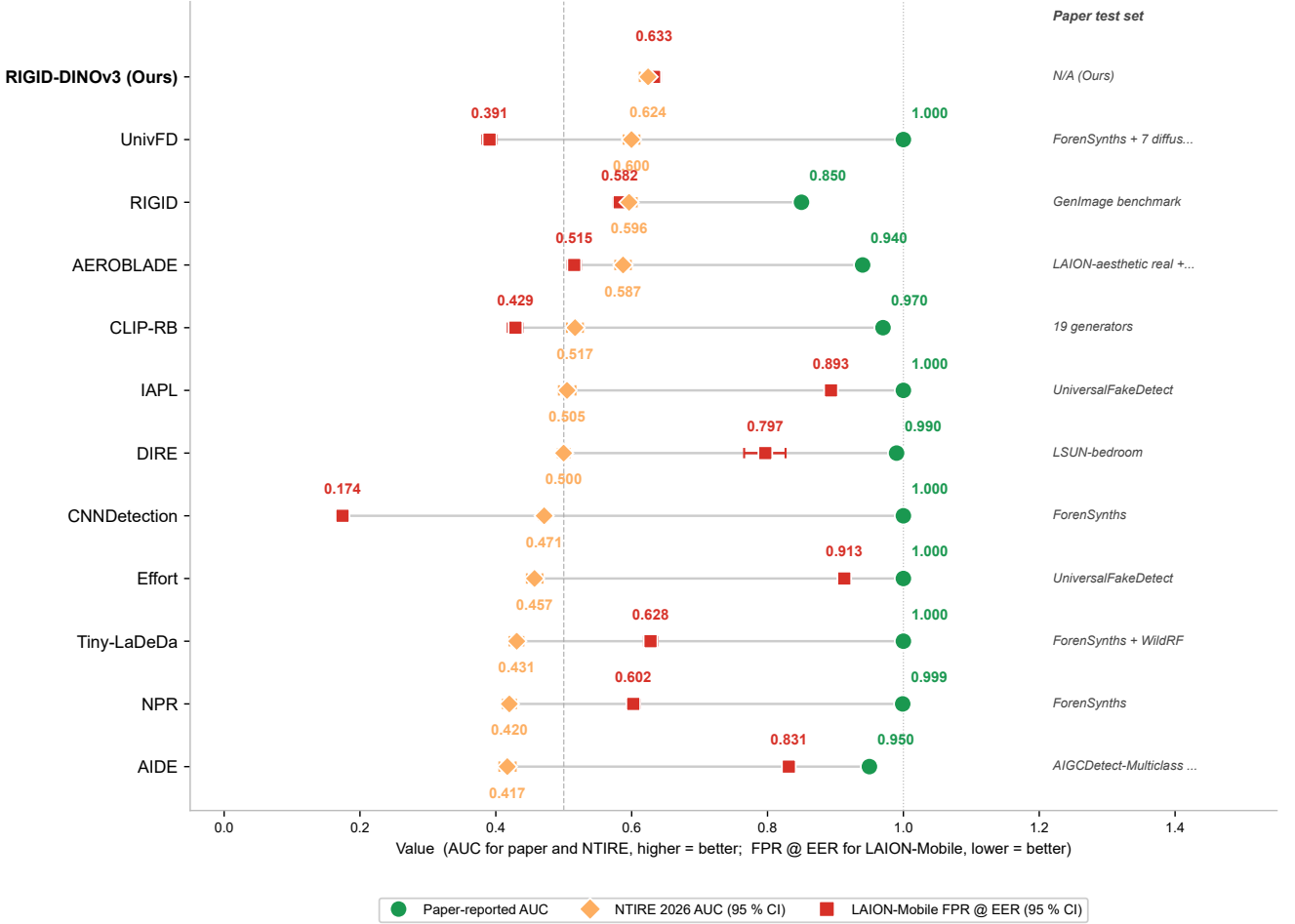
Figure 1: The deepfake-detection reality gap. For each detector, we visualize three different measurements: paper-reported AUC on its own test set (green); NTIRE 2026 AUC [6] (orange, 95% bootstrap CI); and the LAION-Mobile false-alarm rate at the detector’s own NTIRE-calibrated EER threshold (red, n=9,115 , DIRE on 738; the \tau(\text{NTIRE}) column of table 4). Paper-AUC bars are published headlines under each method’s own protocol (context only); directly comparable are the NTIRE and LAION-Mobile columns under our uniform protocol (section 5.1). A deployable detector needs a high NTIRE AUC and a low LAION-Mobile FPR; across the roster the two are mutually exclusive. Results are sorted by descending NTIRE AUC.
