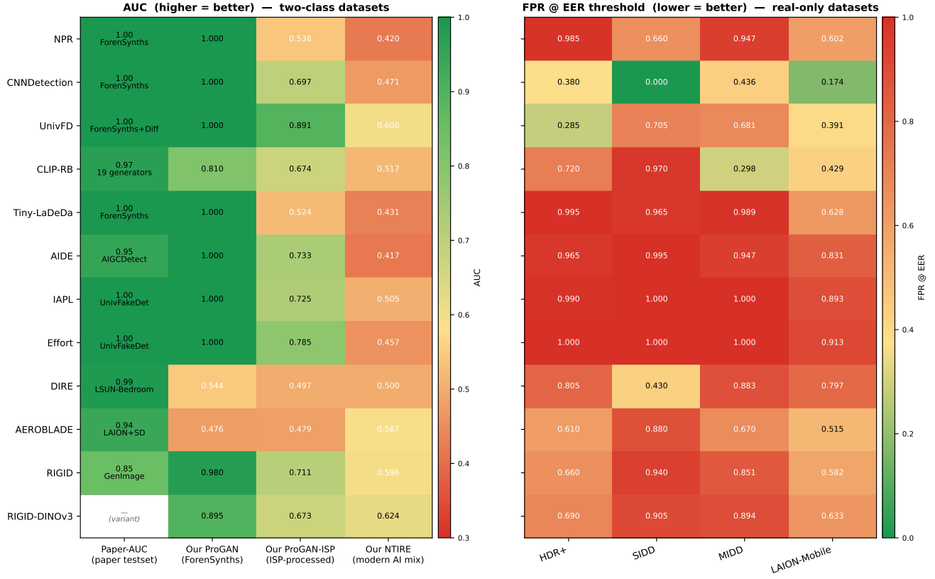
Figure 7: All-datasets matrix. Left : AUC on two-class datasets (higher better): paper-reported, then our ProGAN-ISP and NTIRE 2026. Right : false-positive rate on real-only smartphone/camera datasets at each detector’s NTIRE-calibrated EER threshold (lower better). FPR=0 can reflect a discriminating detector or a default-biased one outputting real unconditionally; the left column disambiguates.
