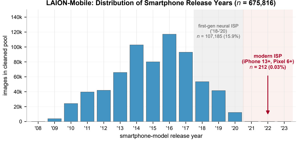
Figure 4: Device-era coverage of the full cleaned LAION-Mobile pool (935,399 images): release-dated images per smartphone-model release year ( n=675,816 release-dated; detector- and threshold-independent). The pool peaks at 2014–2016 hardware and collapses after 2020: only 212 images (0.03%) come from phones released in 2021 or later, so the modern-ISP regime (iPhone 13+, Pixel 6+) the position paper targets is essentially absent. The 2018–2020 heavy bin of section 5.4 is only the first neural-ISP generation.
