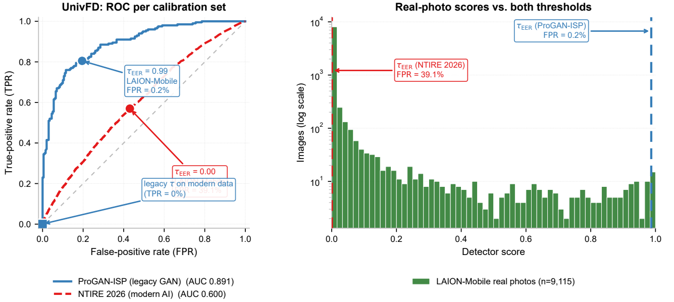
Figure 8: Calibration drift on the best-case detector (UnivFD). Left : ROC curves on the two calibration sets, each EER operating point annotated with the LAION-Mobile false-alarm rate its threshold produces; the square marker projects the legacy threshold onto the modern curve, where it detects essentially nothing. Right : score distribution of the real smartphone photos (log scale) with both EER thresholds. The two defensible calibrations sit at opposite ends of the score range, yielding 0.2% vs. 39.1% FPR on identical photographs.
