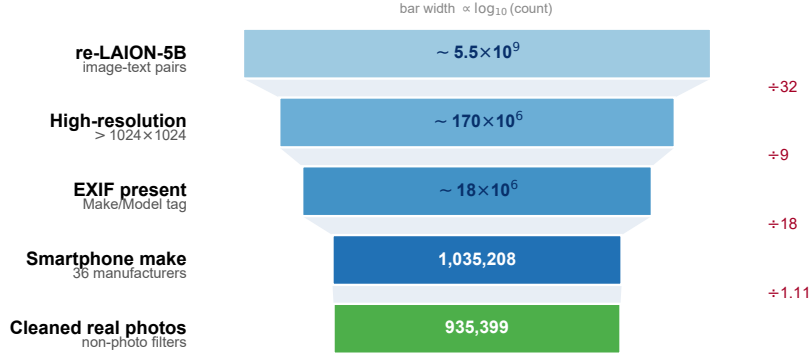
Figure 2: Distillation funnel from re-LAION-5B to the cleaned LAION-Mobile pool. Each tier is annotated with its image count and the reduction factor from the stage above; bar width is proportional to \log_{10}(\text{count}) , as the five stages span four orders of magnitude. The green tier is the 935,399-image cleaned pool from which all evaluation images are drawn (non-photo filtering detailed below).
