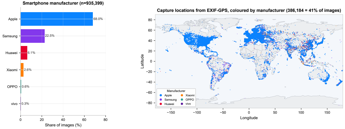
Figure 5: Provenance of the cleaned LAION-Mobile pool ( n=935,399 ). Left : share of images per smartphone manufacturer, each bar in its brand colour. Right : EXIF-GPS capture locations of the geotagged images (386,184, 41.3%), each point coloured by the same manufacturer palette.
