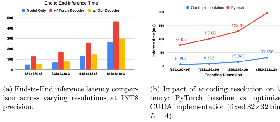
Fig. 3: Latency analysis across implementations and resolutions.
