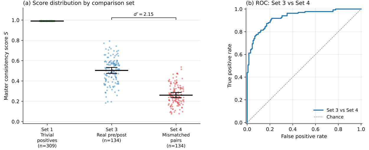
Fig 5 Discriminant performance of the master consistency score S . (a) Per-pair scores by comparison set (Sets 1, 3, and 4). Horizontal bars show set means, and whiskers the 95% bootstrap CI of the mean over resampled source publications. Set 1 has zero within-set variance and carries neither a whisker nor a d' bracket; any d' computed against it rescales a mean difference. Set 2 (sensitivity sweep) is omitted. The bracket gives d' for the primary development contrast, Set 3 versus Set 4 (Section 2.6). (b) Receiver operating characteristic for the same contrast, with Set 3 as the positive class. The empirical area under the curve is 0.928 (95% CI [0.896, 0.959]), against 0.936 predicted by Equation 3.
