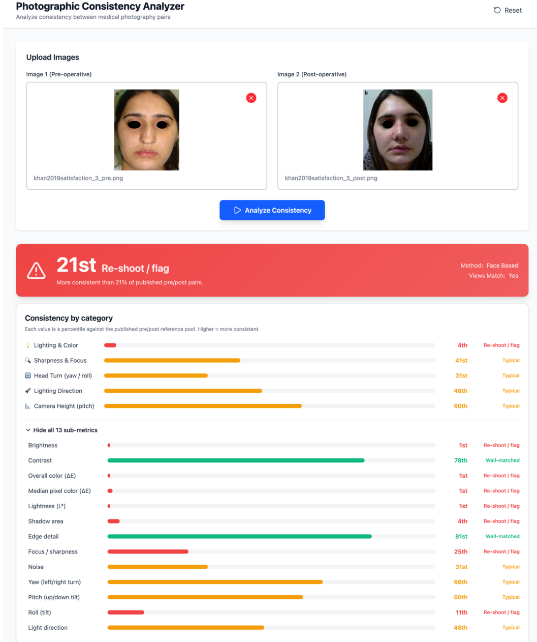
Fig 6 Web interface for the photographic consistency tool, single-pair result view. Scores are shown as percentiles of the Set 3 distribution; the pair illustrated sits at the 21st percentile and is shown as an example of a pair the tool flags. The interface labels the five clusters by their photographic meaning. Against the tags of Table 3, Lighting & Color is C1, Sharpness & Focus is C2, Head Turn is C3, Lighting Direction is C4, and Camera Height is C5. Source pair reproduced under CC BY from. 15
