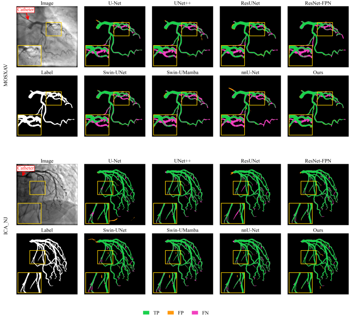
Fig. 3 | Representative segmentation results of different methods on MOSXAV and ICA_NJ. For each dataset, one XCA image and its reference label are shown together with predictions from eight segmentation methods. Green, orange, and magenta denote true positives (TP), false positives (FP), and false negatives (FN), respectively. The red arrows in the XCA images indicate the catheter. The yellow boxes mark connectivity-sensitive regions, which are enlarged in the lower-left corner of each panel.
