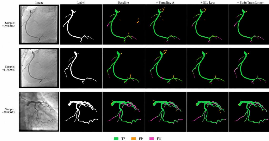
Fig. S1 | Representative visualizations of the single-component ablation study.
