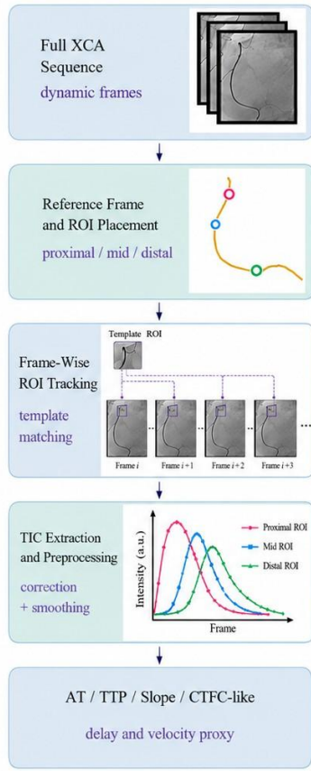
(a) Workflow of Dynamic Contrast-Propagation Analysis
