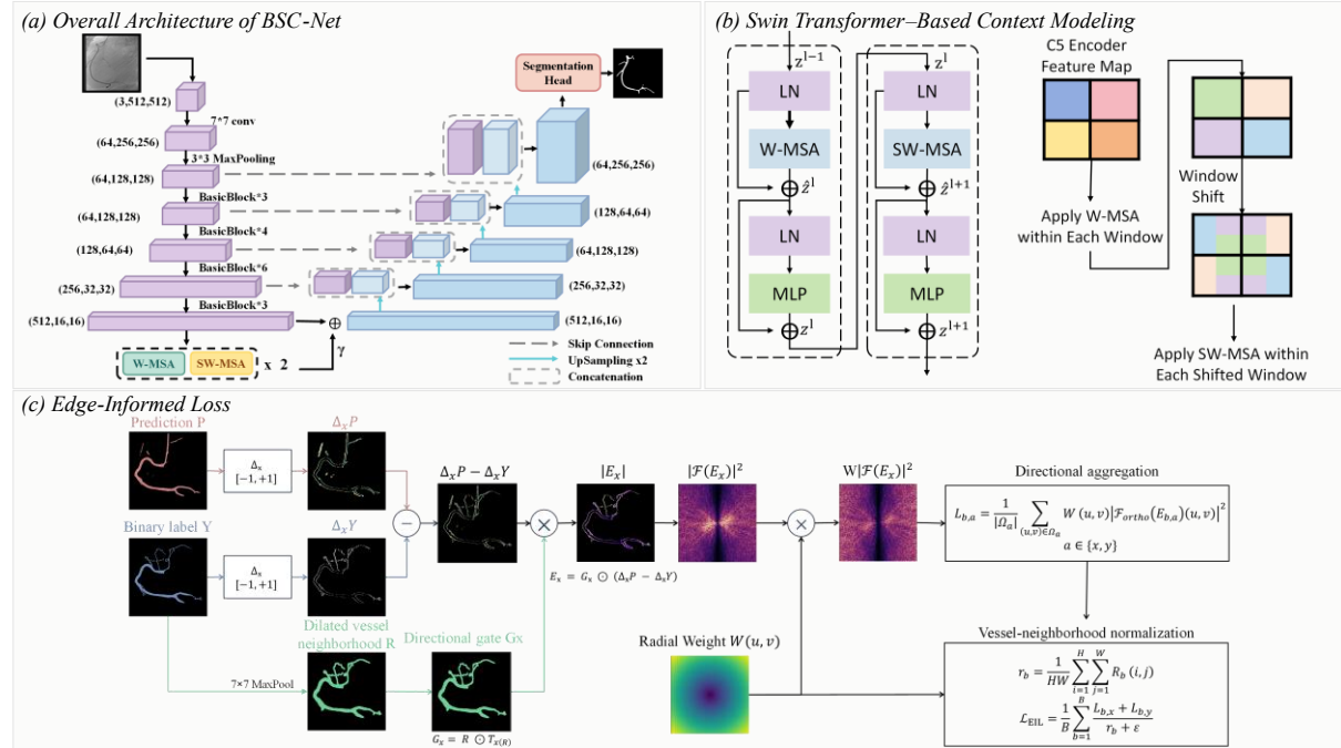
Fig.2 | Network structure of BSC-Net. (a) Overall encoder-decoder architecture of BSC-Net with a Swin Transformer bottleneck. (b) Swin Transformer-based context modeling through W-MSA and SW-MSA. (c) Edge-informed loss (EIL) for enhancing edge consistency and vascular structural continuity.
