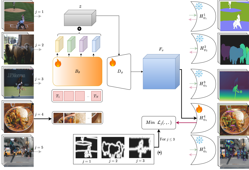
Figure 2. Method Overview. In each iteration, a random vision task—illustrated here with object detection—is selected. After patch tokenization, the backbone processes the tokens, and outputs from four intermediate layers are concatenated to form z . This is then decoded to a shared feature map F_x = D_\phi(z) , which is further processed by the corresponding task-specific projector. For the first three tasks, EDS is applied during loss minimization (*). The gradient-colored backbone highlights layer decay in B_\theta , where later layers receive stronger updates while earlier layers remain more stable, promoting better feature adaptation. Gray/dim arrows indicate inactive tasks, and for task projectors, input and output arrows represent the forward and backward propagation, respectively.
