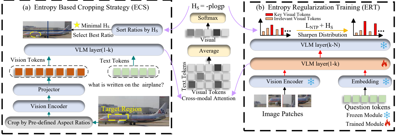
Fig. 2. ENCORE framework. (a) ECS : Compute early-layer cross-modal similarities between visual tokens and prompt, derive prompt-relevant distribution, compute its entropy, select minimal-entropy crop ratio to preserve contiguous prompt-relevant semantics; (b) ERT : During fine-tuning, augment next-token prediction loss with entropy regularizer to encourage sharpening cross-modal attention for accurate key visual token extraction from fragmented high-res inputs.
