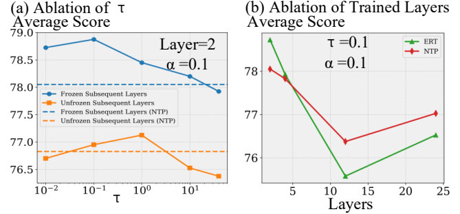
Fig. 4. Ablation study of Entropy Regularization Training (ERT). (a) shows average score on POPE, OCRBench, RWQA and CCBench; In (a)–(b), NTP denotes next-token-prediction fine-tuning.
