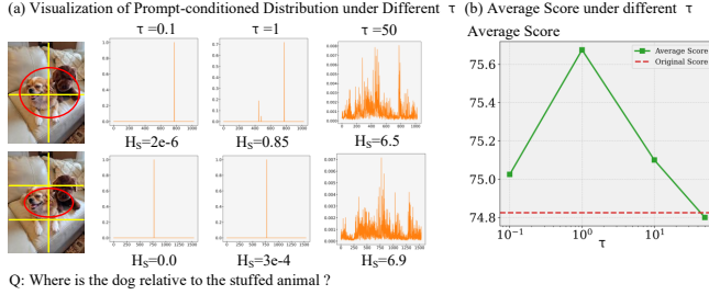
Fig. 3. Ablation study of H_S under varying temperature \tau . (a) Visualization of \tau 's impact. (b) shows the \tau 's impact on average score.
