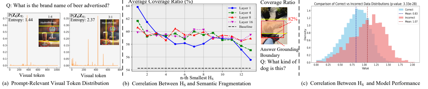
Fig. 1. Insights into image-text entropy. (a) Visualization of prompt-relevant visual-token probability distributions from VLM’s second layer; (b) Images cropped by ratio with the n -th smallest H_S and the maximum IoU(intersection over union) between patches and answer-grounding boundary (baseline: original aspect ratio) on VizWiz [1]. Results show that lower H_S indicates higher coverage ratio, corresponding to more accurate visual understanding; (c) Average H_S distributions over first four layers for correctly answered samples on TextVQA [16], HallB [6], SEED-2 [10], RWQA [20] are lower than that of incorrectly answered samples, with a significantly statistic difference in T-test ( t = -11, p = 3.33 \times 10^{-28} < 0.05 ).
