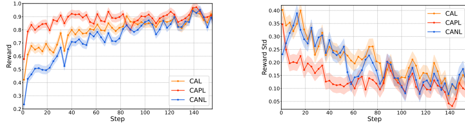
Fig. 10: Left: Reward of CAL, CANL and pure positive learning during training on ScreenSpot-V2. Right: Reward std of CAL, CANL and pure positive learning during training on ScreenSpot-V2.
