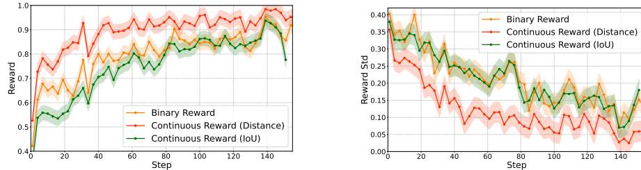
Fig. 9: Left: Reward of binary reward and continuous reward during training on ScreenSpot-V2. Right: Reward std of binary reward and continuous reward during training on ScreenSpot-V2.
