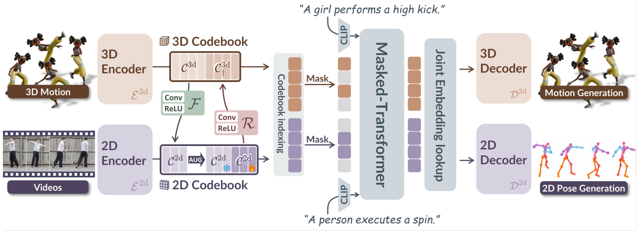
Figure 1: Overview of our MoVT. We first train a 3D Residual VQ-VAE on 3D motion data, and learn the bidirectional mapping networks ( \mathcal{F} and \mathcal{R} ) between the 3D codebook C^{3d} (base level of Residual VQ-VAE) and 2D codebook C^{2d} . Next, the 2D codebook is frozen and augmented on large-scale video motion data to obtain C^{2d}_+ , which is mapped back to the 3D domain via \mathcal{R} as C^{3d}_+ and merged with the original 3D codebook. The 3D encoder-decoder is then fine-tuned to adapt to the enriched codebook. Finally, a masked transformer is trained on motion token sequences from both 3D and 2D video datasets, allowing the generator to produce 3D motion and 2D poses.
