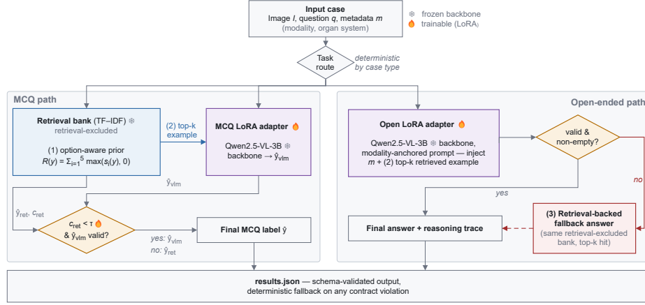
Fig. 1. Inference pipeline. Task type is dispatched deterministically, and one retrieval-excluded TF-IDF bank is used three ways: (1) an option-aware decision prior \hat{y}_{ret}, c_{ret} for the MCQ confidence gate; (2) k in-prompt retrieved examples for both adapted VLMs ( k = 1 during adapter training, k = 3 in the submitted runtime); (3) a retrieval-backed fallback answer (dashed), only when OE generation violates the output contract.
