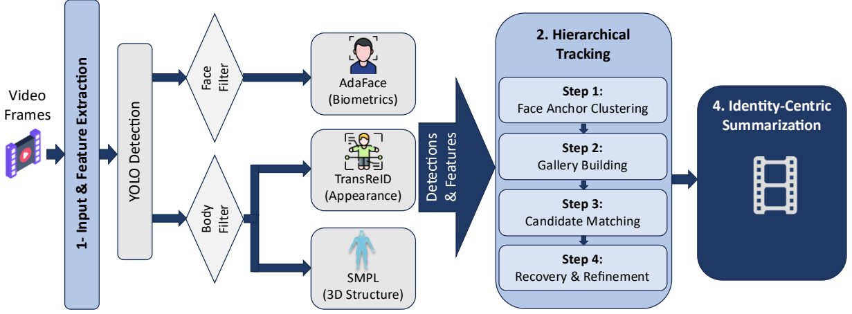
Figure 1: Overview of the proposed hierarchical tracking and summarization framework. The pipeline begins by extracting features from video frames, where quality filters are applied before computing the AdaFace (biometrics), TransReID (visual appearance), and SMPL (3D body shape) embeddings. The tracking process consists of four hierarchical steps: (1) Face Anchor Clustering uses DBSCAN on high-quality faces to find unique identities; (2) Gallery Construction establishes a robust profile for each cluster; (3) Candidate Matching links the remaining detections (e.g., occluded or back-turned) to these profiles; and (4) Recovery and Refinement handles unmatched tracklets and smooths the trajectories. Finally, the system generates an Identity-centric summary containing selected keyframes and metadata for each person.
