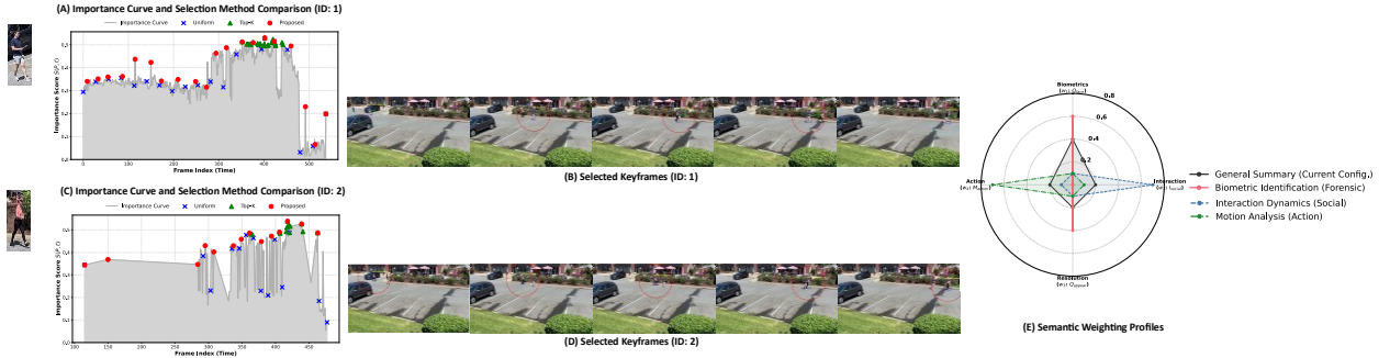
Figure 3: Qualitative evaluation of summary selection strategies for two distinct identities. (A, C) Temporal evolution of the importance score S(P, t) for ID 1 and ID 2, respectively. Our proposed method (red circles) effectively captures semantically rich frames while maintaining temporal diversity, avoiding the severe redundancy of the Top-K baseline (green triangles) and the suboptimal semantic performance of Uniform sampling (blue crosses). (B, D) The resulting visual summaries generated by the proposed method, demonstrating a complete and diverse narrative sequence for each identity. (E) Semantic profiles illustrating the system's ability to generate query-guided summaries, enabling the dynamic creation of personalized summaries based on specific analytical intents.
