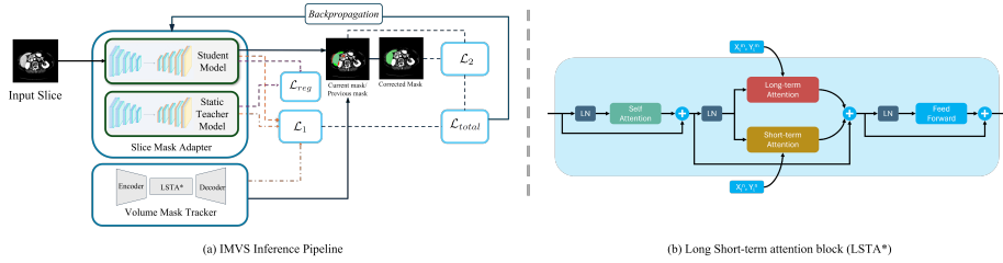
Fig. 1. Overview of the IMVS closed annotation loop. The SMA predicts a mask the user refines with scribbles (teacher–student online adaptation); the frozen VMT propagates the corrected mask across adjacent slices via long/short-term attention and a memory bank.
