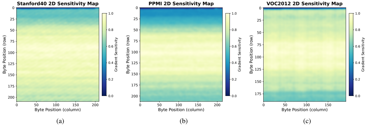
Figure 3: Two-dimensional gradient sensitivity maps on (a) Stanford40, (b) PPMI, and (c) VOC2012 Action. The one-dimensional byte-level sensitivity sequence is reshaped into a two-dimensional matrix. Spatially coherent patterns indicate that the bitstream preserves an implicit two-dimensional structure inherited from the JPEG encoding order.
