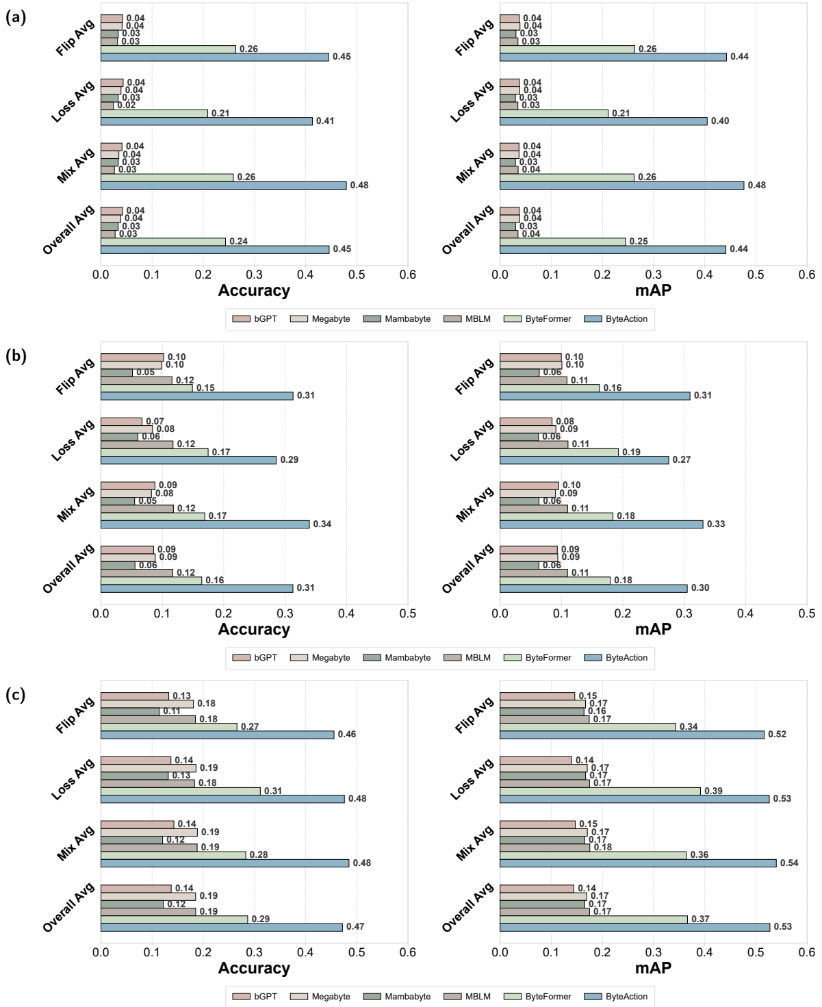
Figure 4: Comparison of bitstream-domain methods by corruption type on (a) Stanford40, (b) PPMI, and (c) VOC2012 Action. Each group reports the average Accuracy (left) and mAP (right) across four severity levels within the corresponding corruption type (Flip, Loss, Mixed) and overall.
