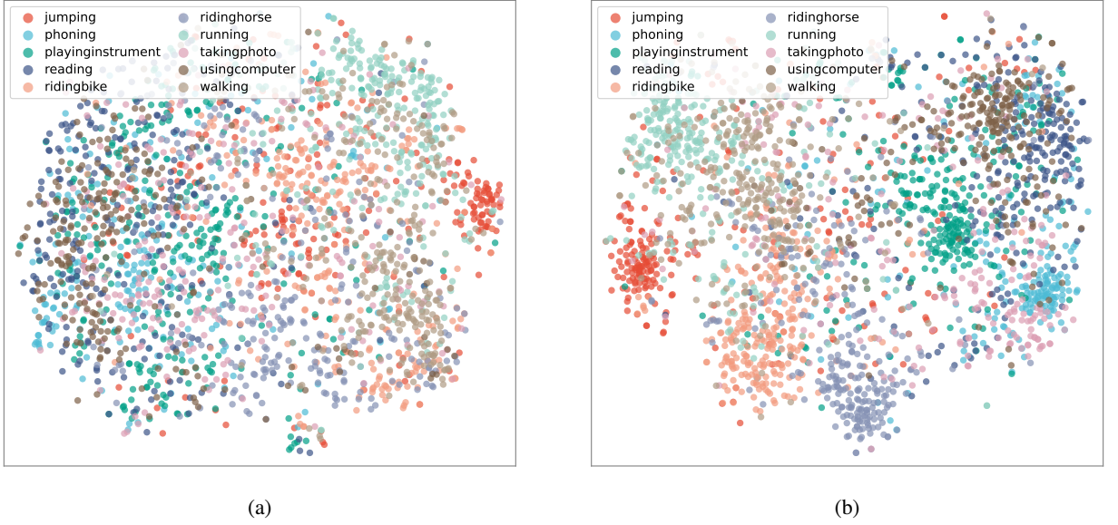
Figure 5: t-SNE visualization of learned features on VOC2012 Action (10 classes) under corruption. (a) ByteFormer. (b) ByteAction (Ours). Best viewed in color.
