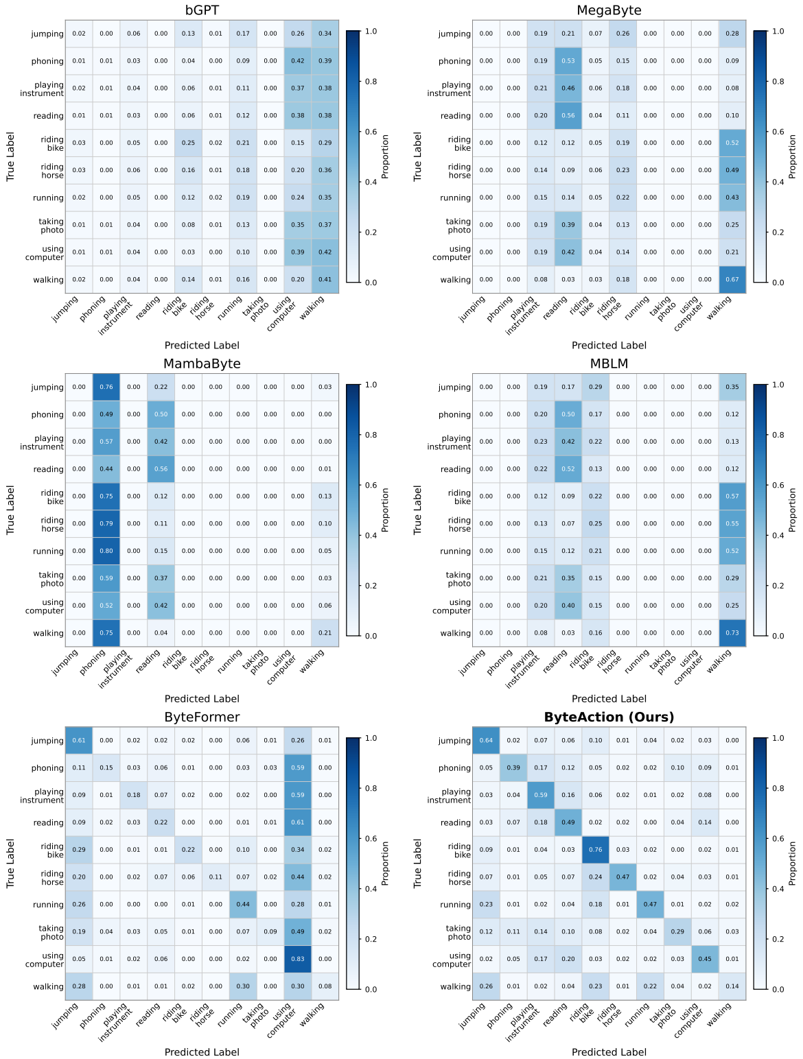
Figure 6: Confusion matrices of bitstream-domain methods on VOC2012 Action, averaged over all 12 corruption scenarios.
