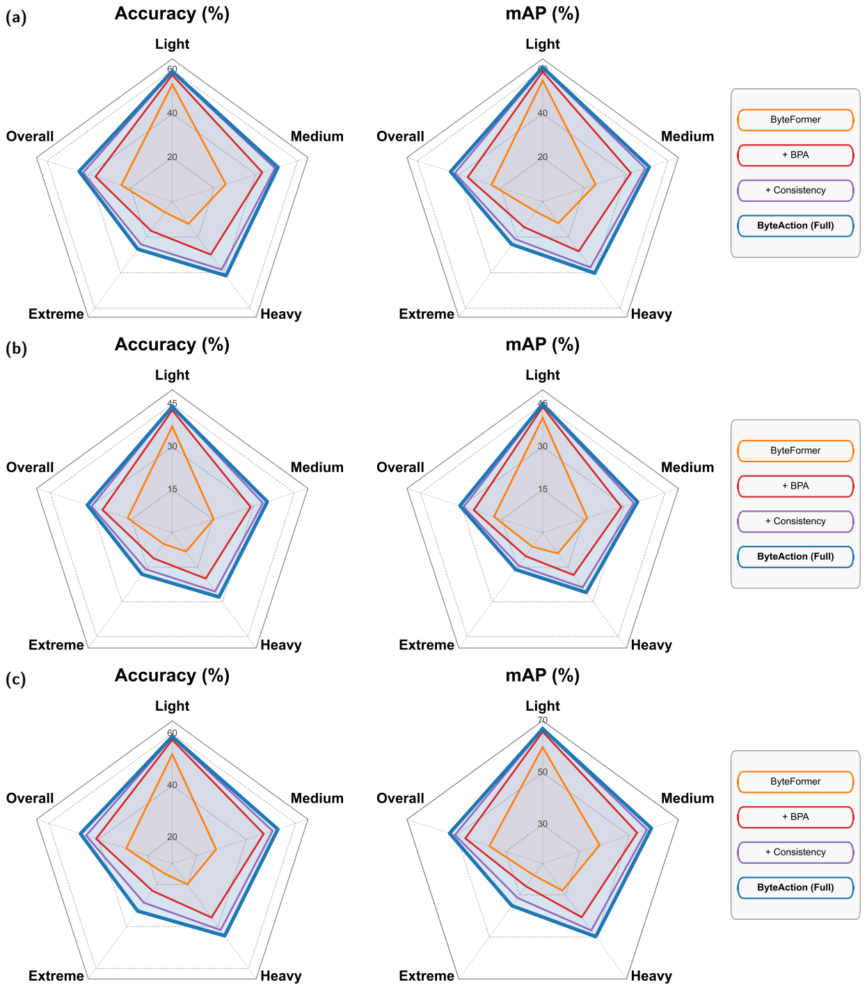
Figure 7: Ablation study on the proposed components across (a) Stanford40, (b) PPIM, and (c) VOC2012 Action. Each axis represents the average performance at a given corruption severity level (Light, Medium, Heavy, Extreme) and the overall Corrupt Average. Left: Top-1 Accuracy (%). Right: mAP (%). Larger coverage area indicates stronger robustness.
