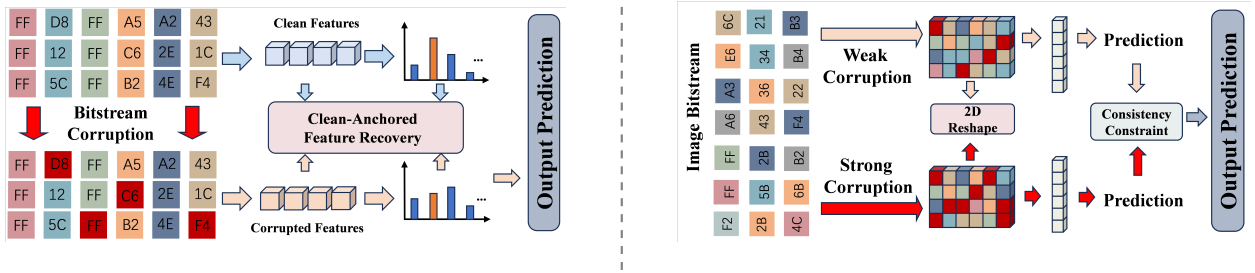
Figure 1: Comparison of two bitstream-domain pipelines for action recognition under bitstream corruption. (a) The existing approach aligns corrupted features with intact features through a frozen teacher model. (b) The proposed ByteAction reshapes byte sequences into two-dimensional matrices via BPA and enforces prediction consistency between two corruption levels without requiring a teacher model.
