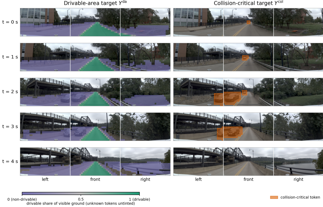
Figure 4: Example of ground-truth affordance targets at t = 0 –4 s.
