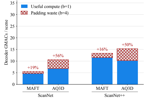
Figure 7. Cost of padding a batch to its largest query set. Solid bars are the unpadded per-scene cost measured at batch size 1; hatched bars are the additional arithmetic resulting from batch size 4, annotated as a percentage of the unpadded cost. A fixed budget admits no query-side padding, so MAFT’s residual growth comes entirely from the varying superpoint count N_S , which both methods share.
