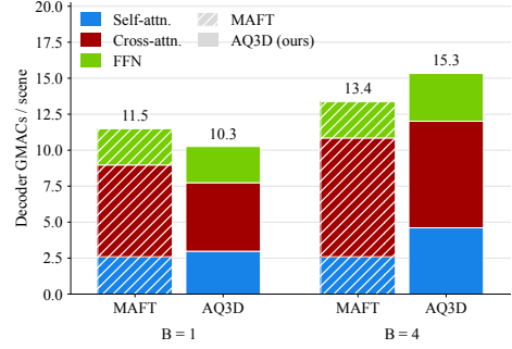
Figure 6. Decoder compute on ScanNet++V2 , plotted as in Fig. 5. MAFT uses N_Q = 800 . At an average query budget equal to the baseline’s, the adaptive decoder is cheaper overall. Relying on RoPE alone removes the concatenated positional channel from the query-key product, which offsets the higher self-attention cost from a variable N_Q .
