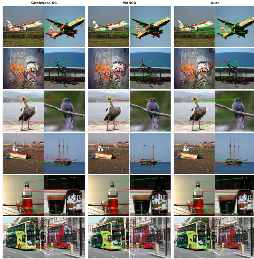
Fig. 4: Additional results on SPair-71k across object categories.
