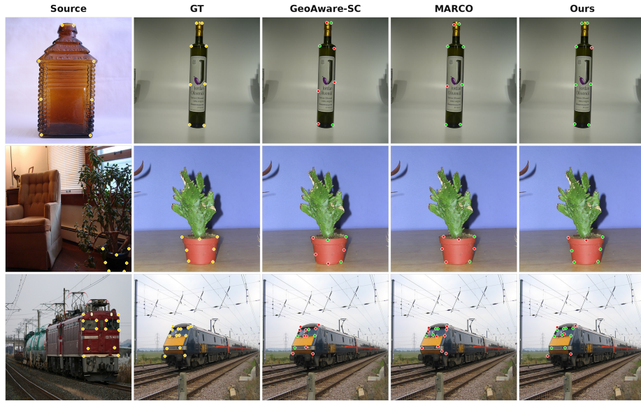
Fig. 3: Qualitative comparison on SPair-71k (PCK@0.01, per-image). Green and red dots indicate correct and incorrect correspondences, respectively. While GeoAware-SC and MARCO capture the approximate location of most keypoints, they tend to deviate slightly from the ground truth under the fine-grained threshold. In contrast, ImCorr matches the same keypoints with substantially higher precision.
