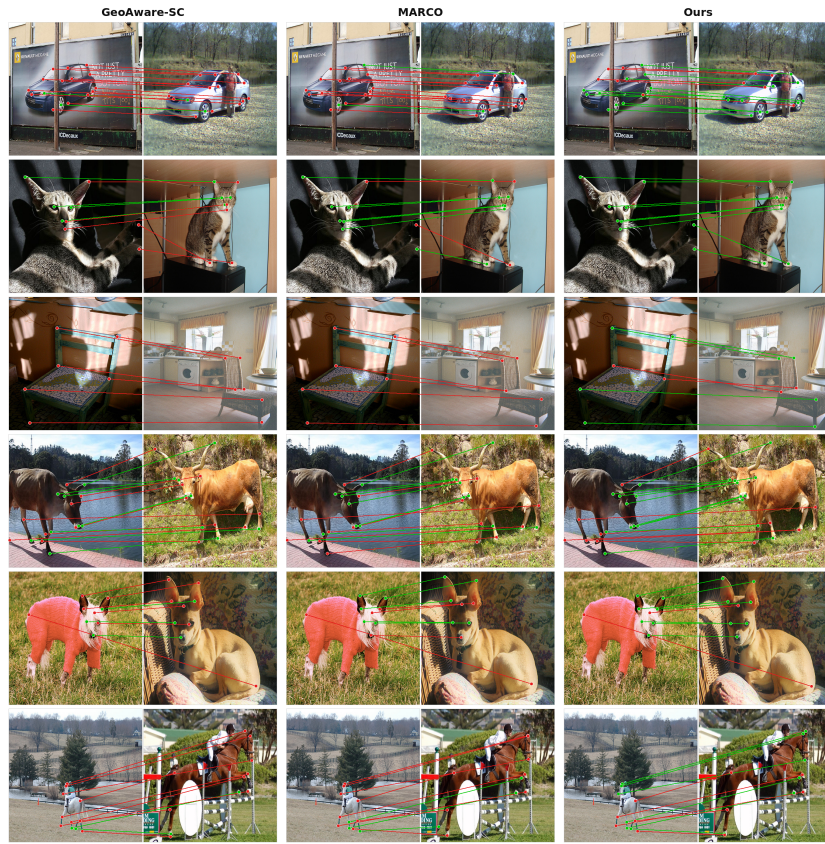
Fig. 5: Additional results on SPair-71k across object categories.
