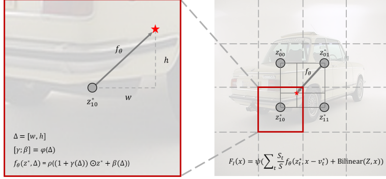
Fig. 2: Overview of the FiLM-conditioned decoder and local ensemble. (Left) Zoomed-in view of the decoding process for grid point z_{10}^* : the offset \Delta = [w, h] relative to the query coordinate is transformed by an MLP \varphi into channel-wise modulation parameters [\gamma; \beta] (Eq. (5)), which modulate the grid feature (Eq. (6)) and are subsequently refined by a nonlinear rendering MLP \rho to produce the per-grid-point feature f_\theta(z^*, \Delta) (Eq. (7)). (Right) The four per-grid-point features surrounding the query coordinate (red star) are combined via area-based weighting, added to a bilinear residual, and projected through a linear layer \psi to produce the final feature F_I(x) (Eq. (8)).
