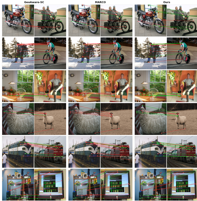
Fig. 6: Additional results on SPair-71k across object categories.
