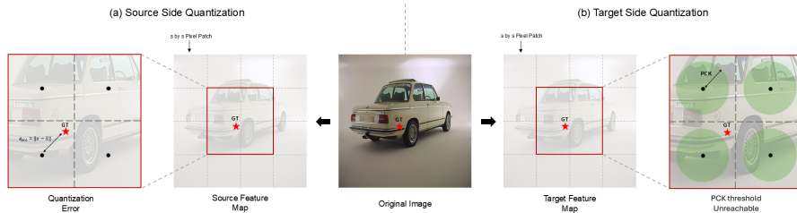
Fig. 1: Illustration of grid quantization error in semantic correspondence. (a) Source-side quantization: the same patch feature is used in matching regardless of where within the patch a keypoint lies, so the keypoint’s exact positional information is not reflected in the representation. The distance to the nearest patch center, \|\mathbf{x} - \hat{\mathbf{x}}\| , quantifies the extent of positional information disregarded. (b) Target-side quantization: when the ground-truth location falls between grid points, no grid feature represents its precise location, making correct localization structurally impossible within the PCK threshold.
