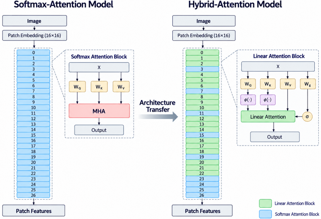
Figure 9: Architectural overview of the softmax and hybrid attention models.
