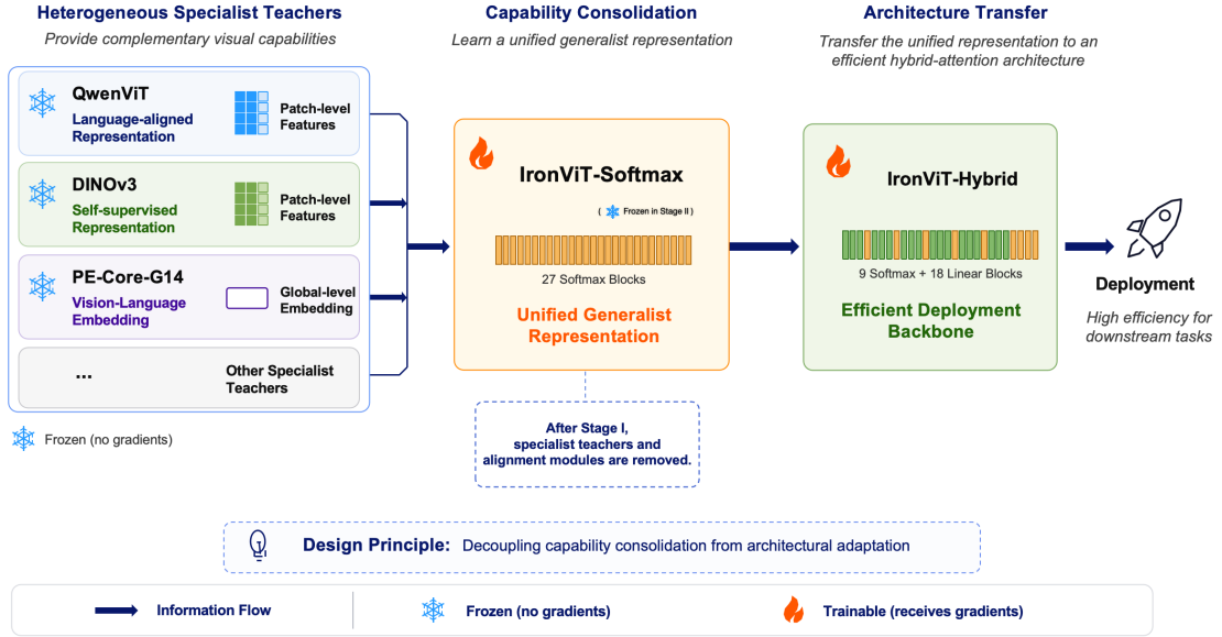
Figure 6: Overview of IronViT. Stage I consolidates complementary specialist capabilities into a softmax attention bridge, and Stage II transfers the unified representation to a hybrid attention encoder through progressive distillation.
