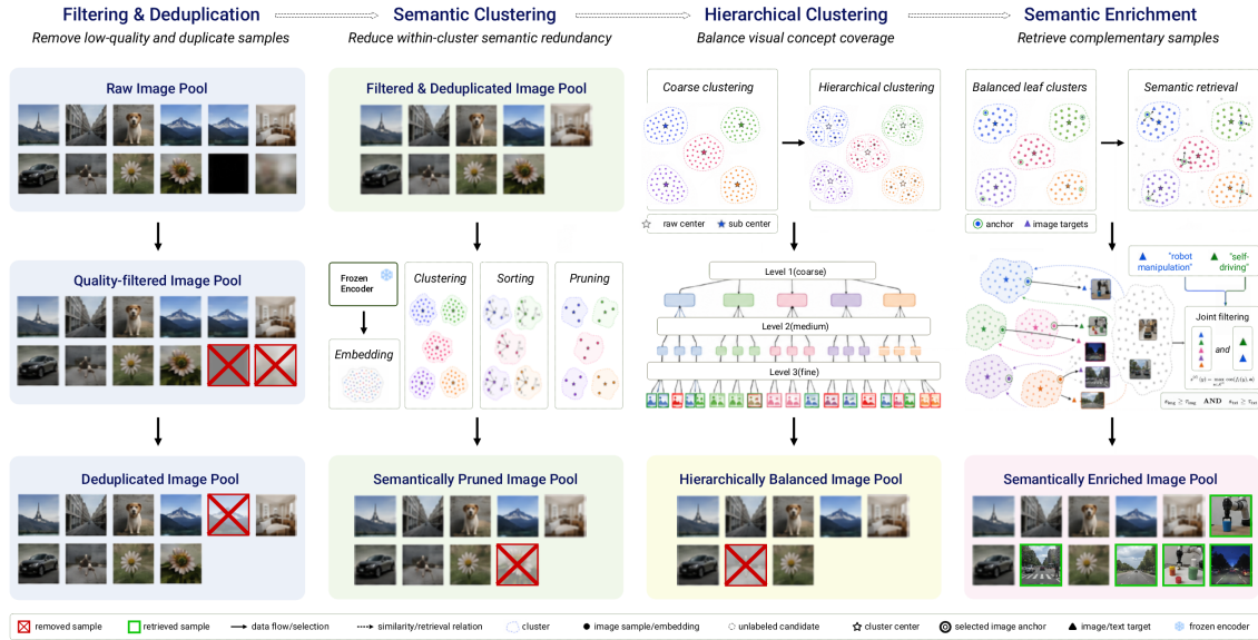
Figure 2: Overview of the proposed data curation framework.
