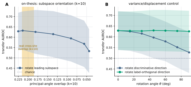
Fig. 5. Controlled rotation of subspace orientation, on the six largest ABIDE sites ( n_s \geq 42 ; 10 split-halves per site, seven rotation angles 0^\circ – 90^\circ ). (A) On-the-sites test: rotating the leading effective subspace ( k = 10 ) drives source–target overlap down and degrades transfer AUROC monotonically toward chance; the shaded vertical band marks the empirical ABIDE overlap. (B) Variance/displacement control: rotating the discriminative direction degrades transfer, whereas rotating a label-orthogonal direction of matched displacement ( \|\Delta x\| = 6.82 ) does not. The rotation is orthogonal and restores the site mean, preserving the feature mean and the covariance eigenvalue spectrum (changes \sim 10^{-15} and \sim 10^{-13} ), so only orientation is perturbed. Bands denote \pm SD across sites and split-halves; effect sizes and the per-site test are reported in the text.
